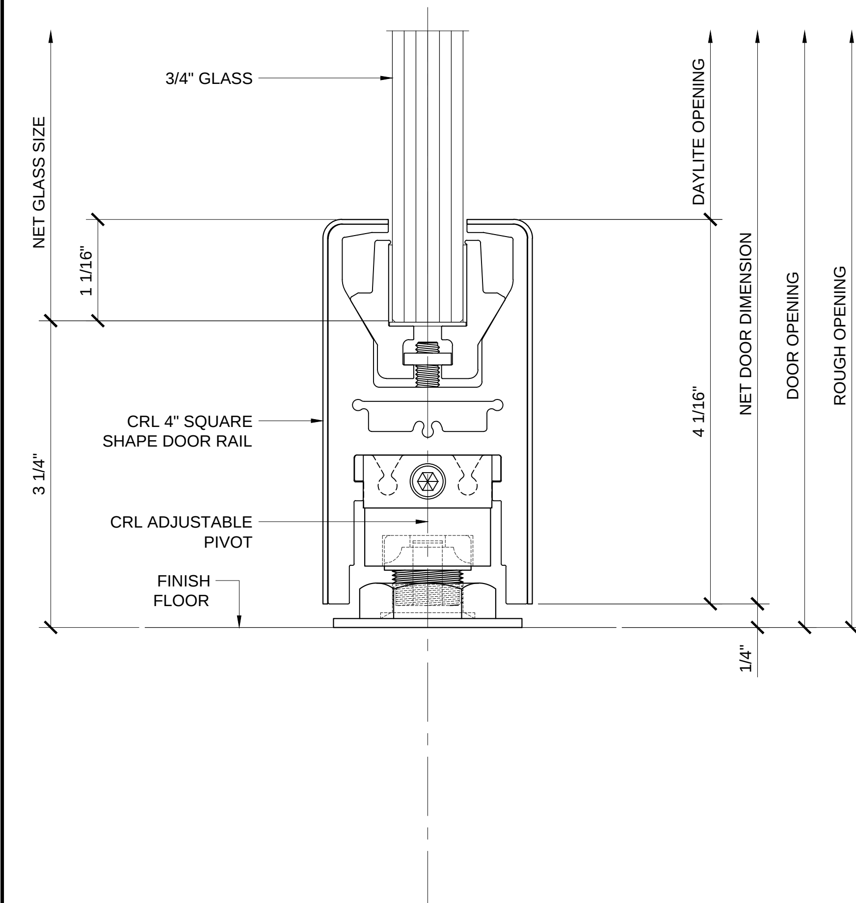
SECTION DETAIL @ SILL
