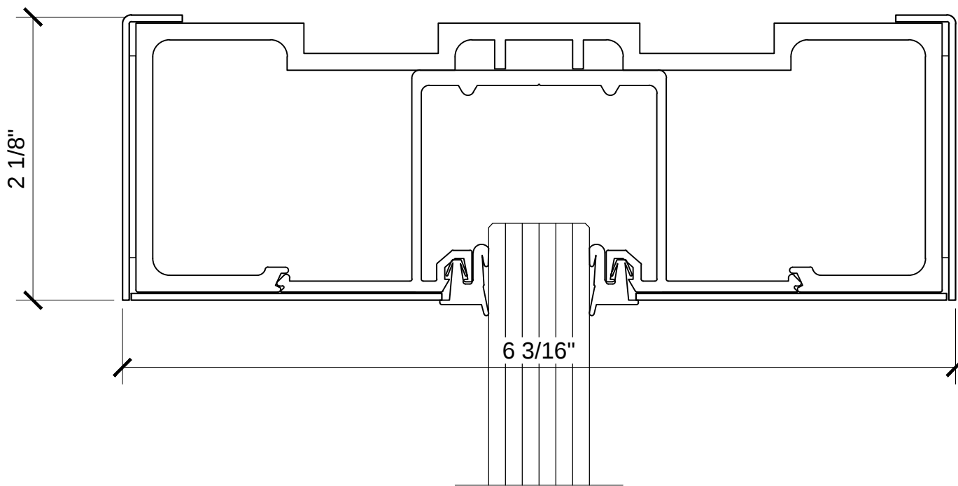
2" x 6" CLAD HEADER W/ GLAZING POCKET DCH6 SERIES
