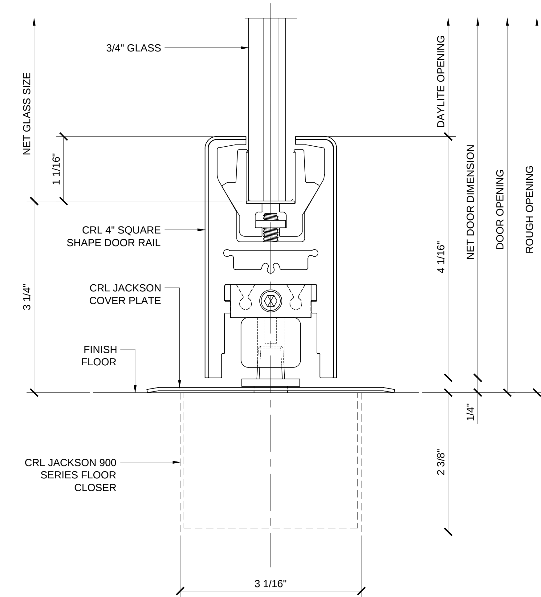
SECTION DETAIL @ DOOR SILL (2.6)
