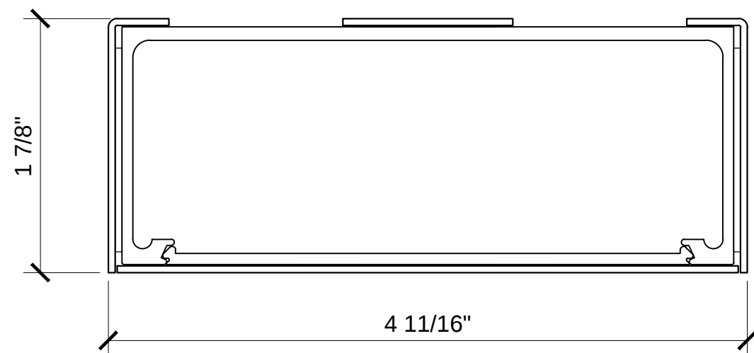
1 3/4" x 4 1/2" CLAD HEADER DCH SERIES
