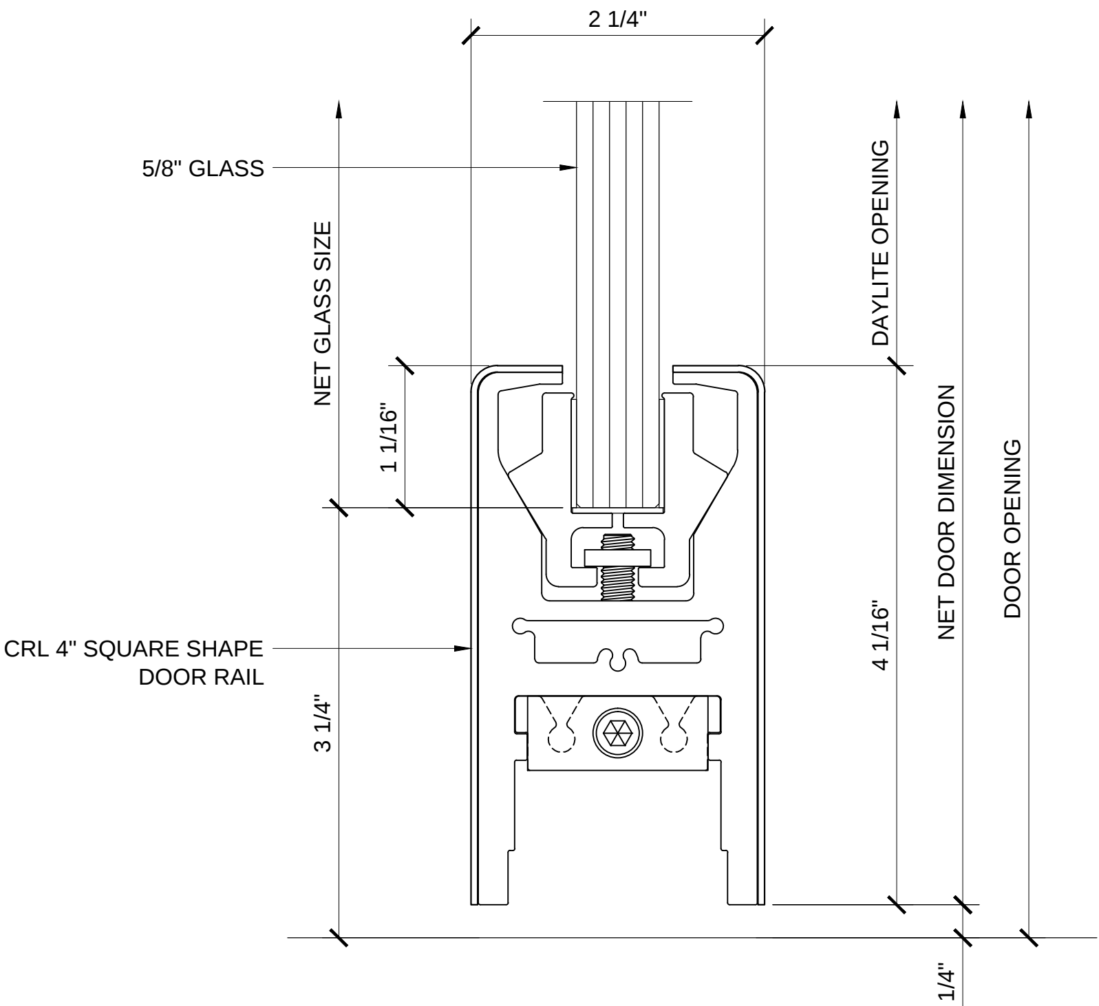
CRL DR4S58 4" TALL SQUARE DOOR RAIL
