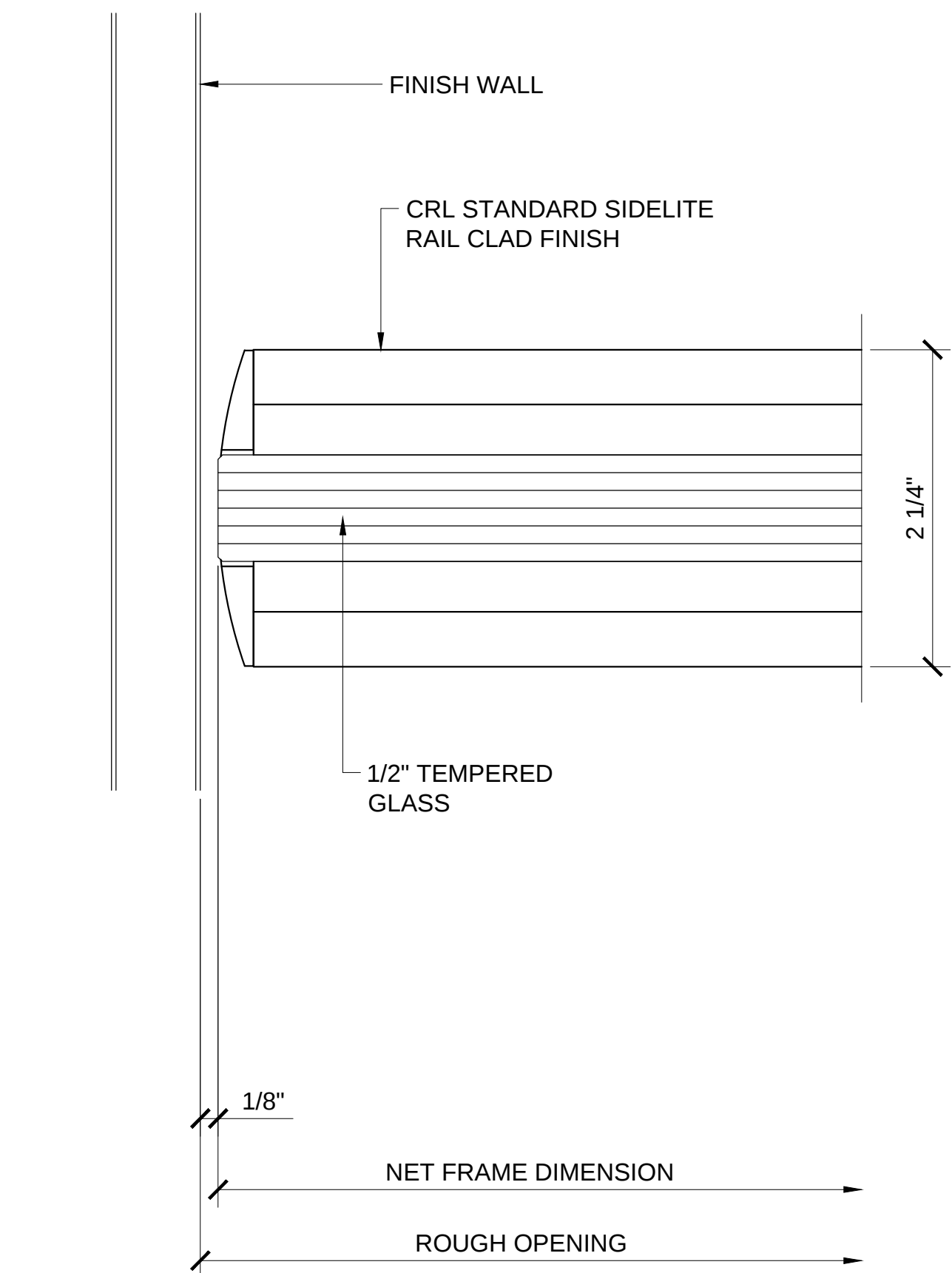
PLAN VIEW @ SIDELITE JAMB (2.7)
