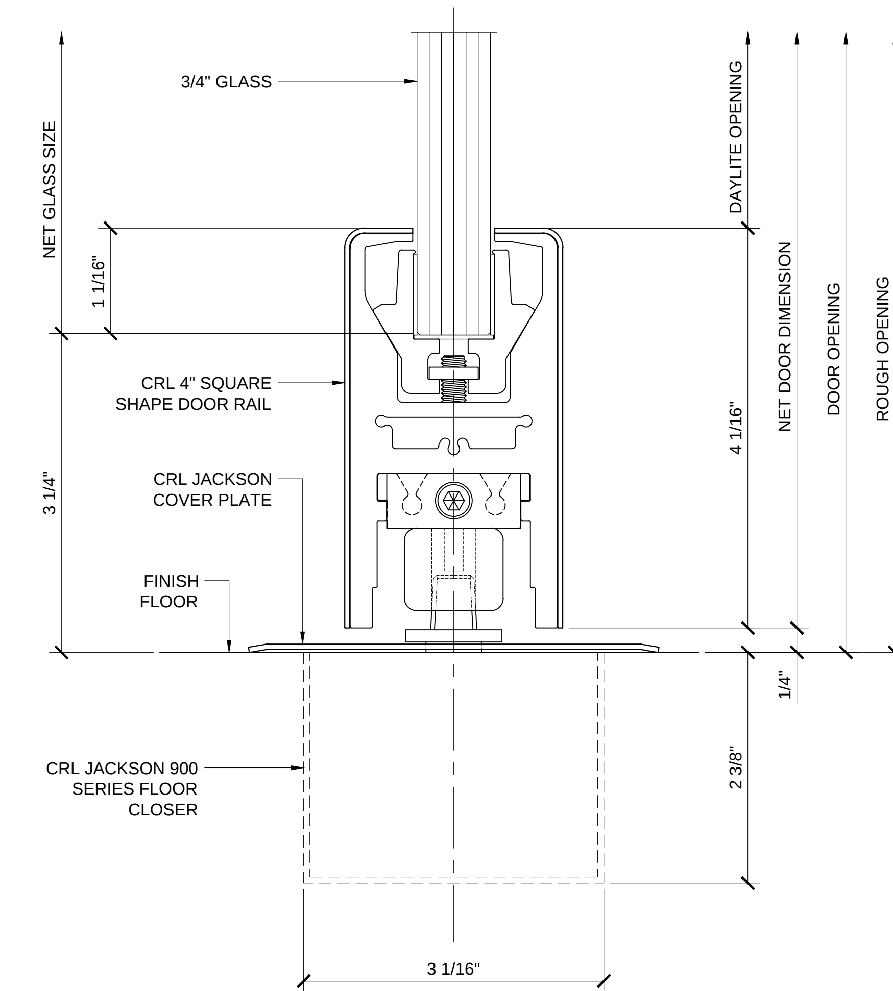
SECTION DETAIL @ SILL
