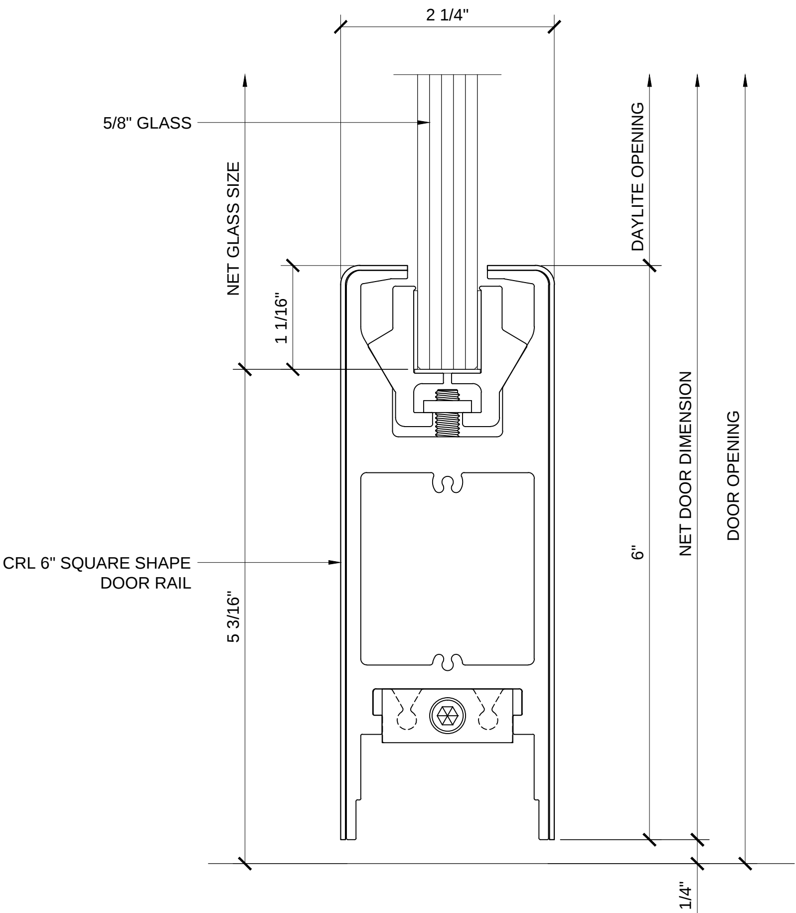
CRL DR6S58 6" TALL SQUARE DOOR RAIL
