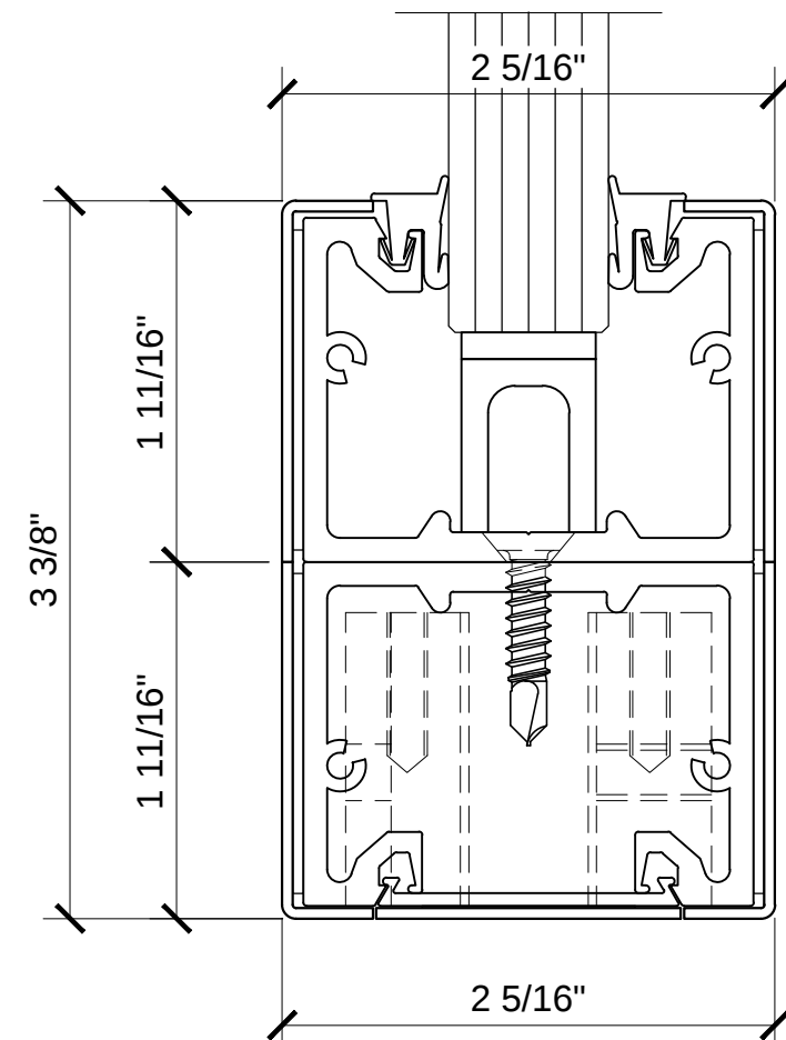
NARROW CLAD FLOATING HEADER 3NFH SERIES
