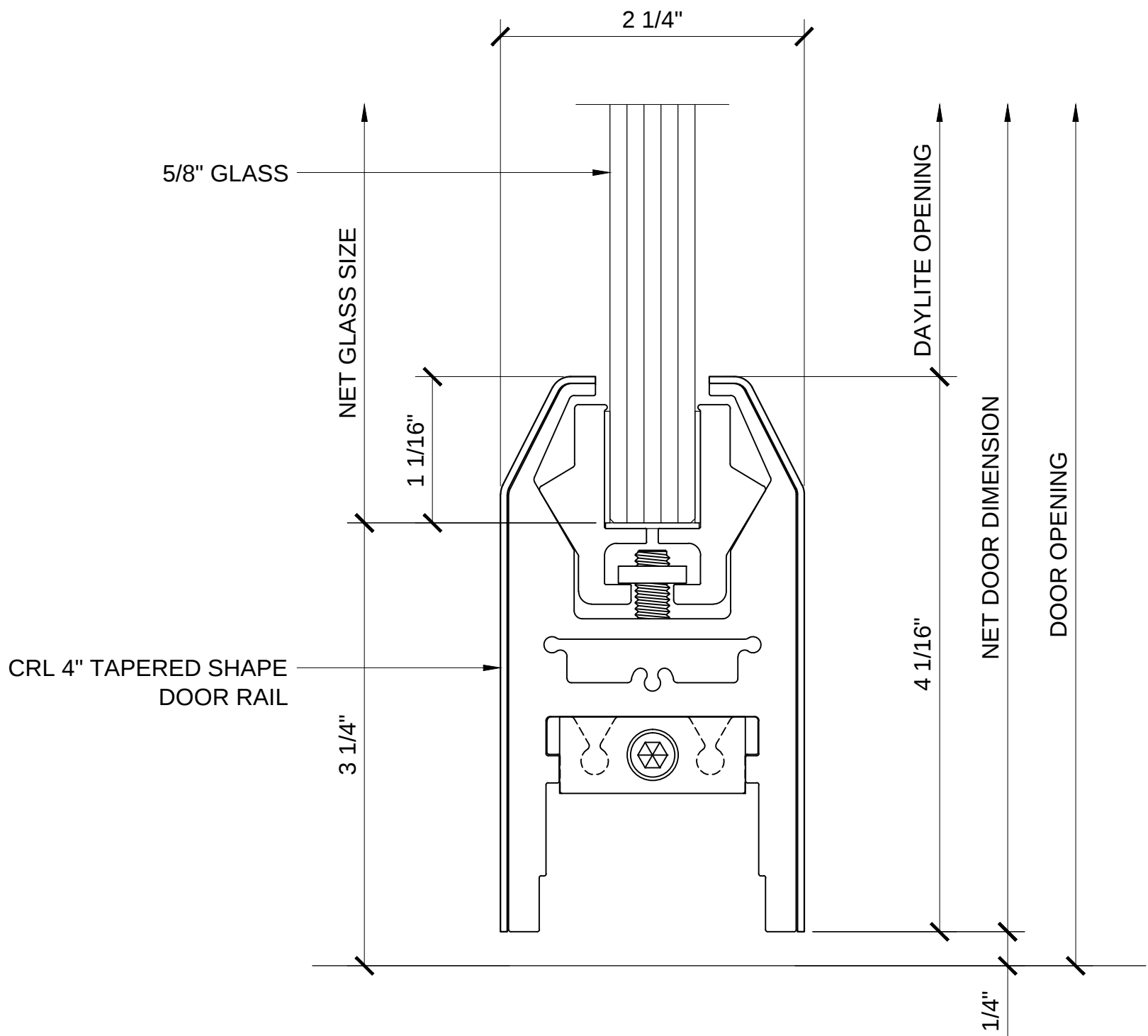
CRL DR4T58 4" TALL TAPERED DOOR RAIL
