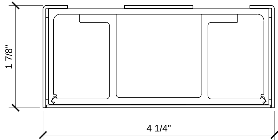
1 3/4" x 4" CLAD HEADER W/ HARDWARE ADAPTOR DCH4 SERIES
