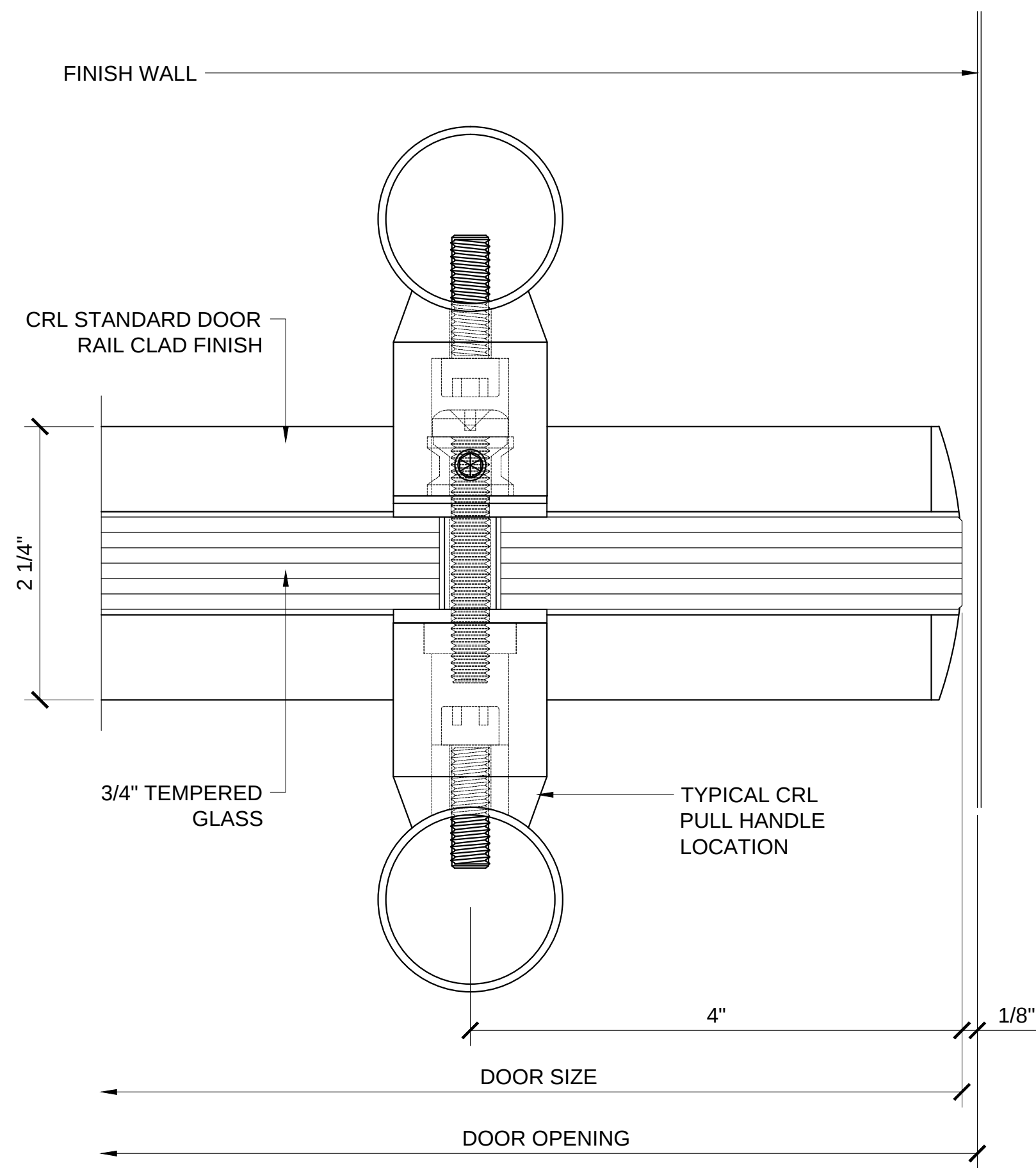
PLAN VIEW @ JAMB
