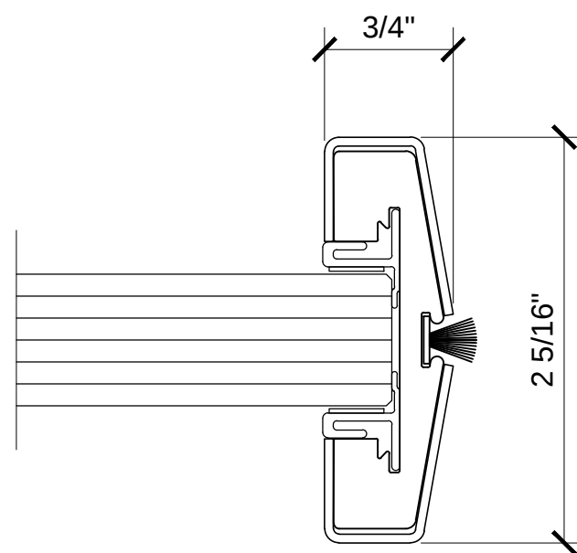
3/4" x 2 5/16" CLAD VERTICAL STYLE W34 SERIES
