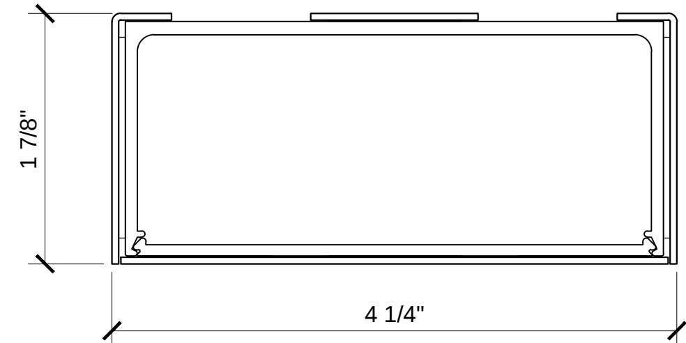
1 3/4" x 4" CLAD HEADER DCH4 SERIES
