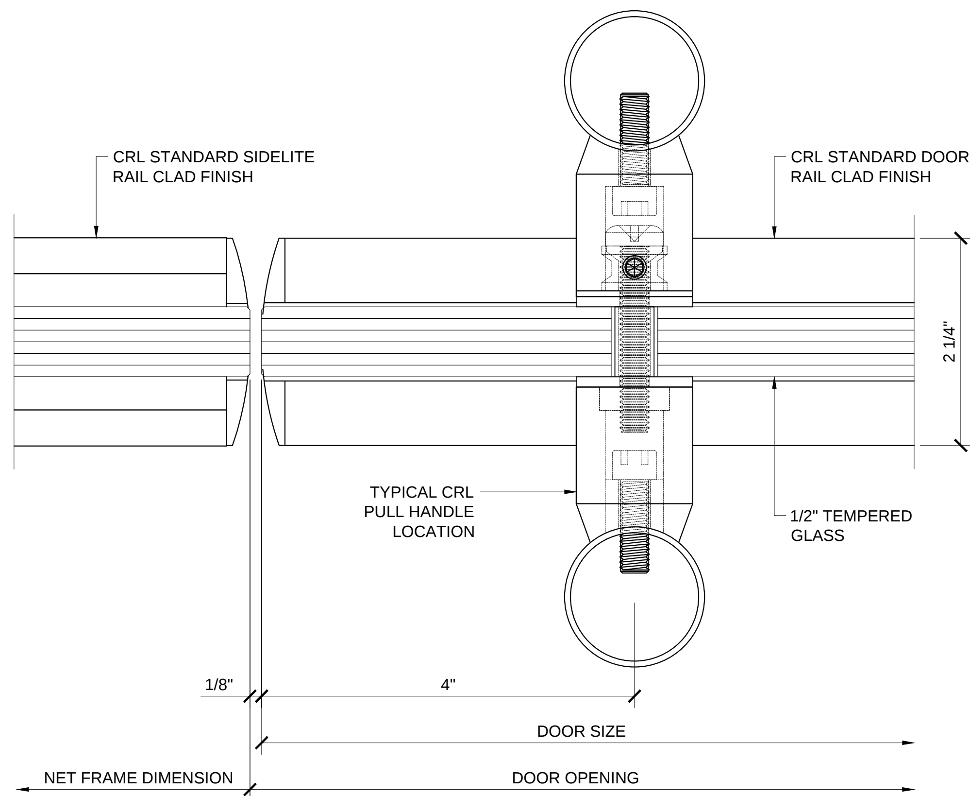
PLAN VIEW @ SIDELITE /DOOR JAMB (2.10)
