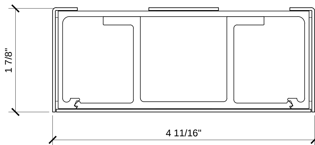
1 3/4" x 4 1/2" CLAD HEADER W/ HARDWARE ADAPTOR DCH SERIES
