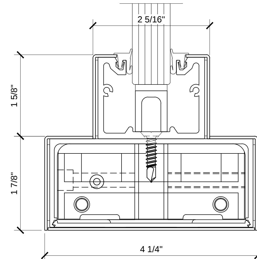
1 3/4" x 4" CLAD FLOATING HEADER DCH4 SERIES
