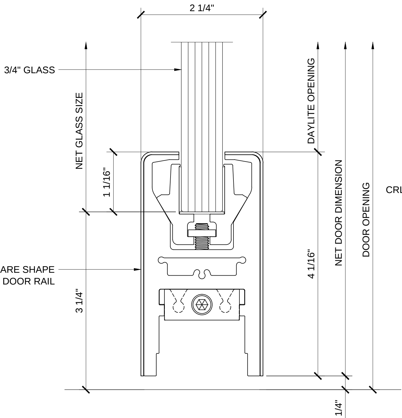
CRL DR4S34 4" TALL SQUARE DOOR RAIL
