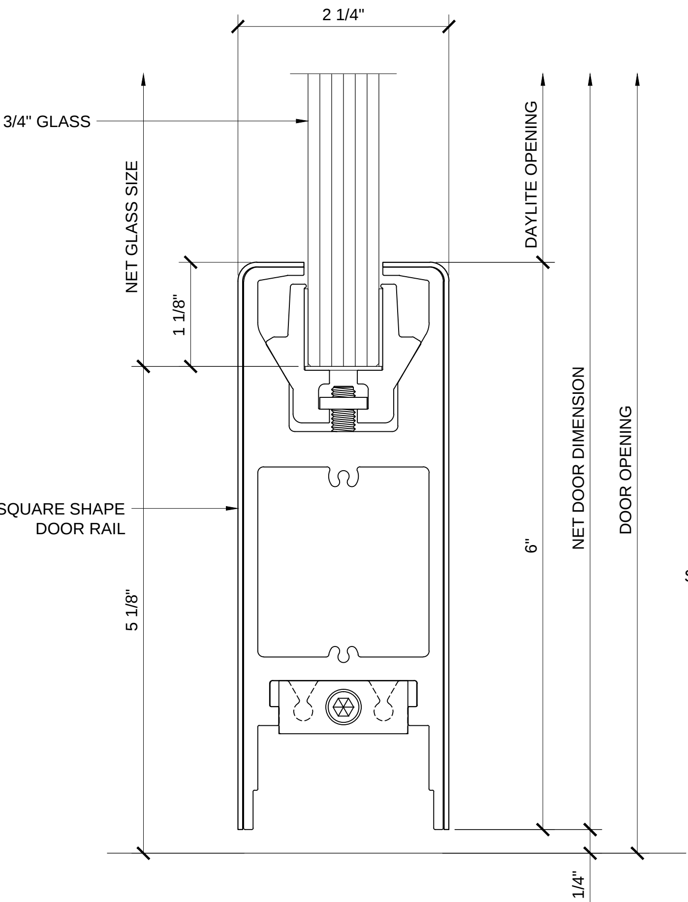
CRL DR6S34 6" TALL SQUARE DOOR RAIL
