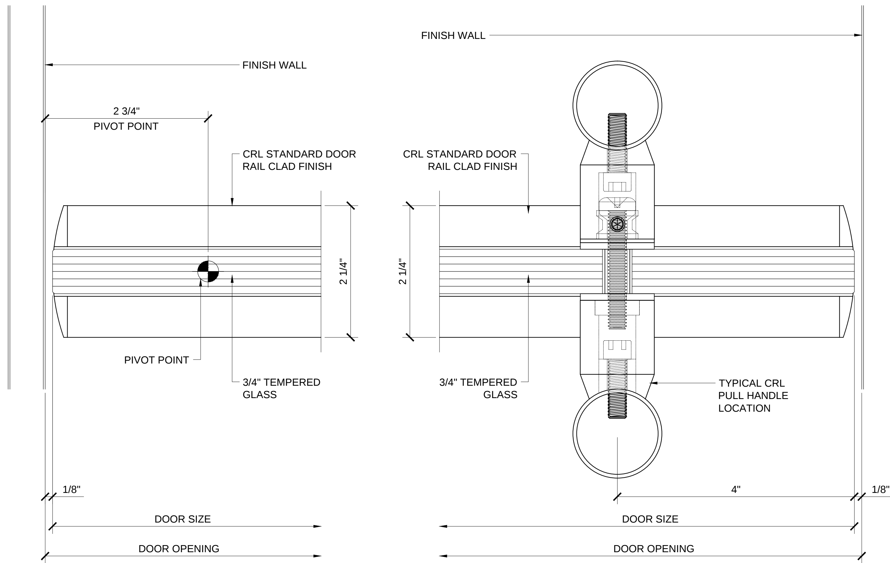
PLAN VIEW @ JAMB
