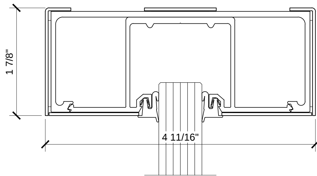
1 3/4" x 4 1/2" CLAD HEADER W/ GLAZING POCKET DCH SERIES
