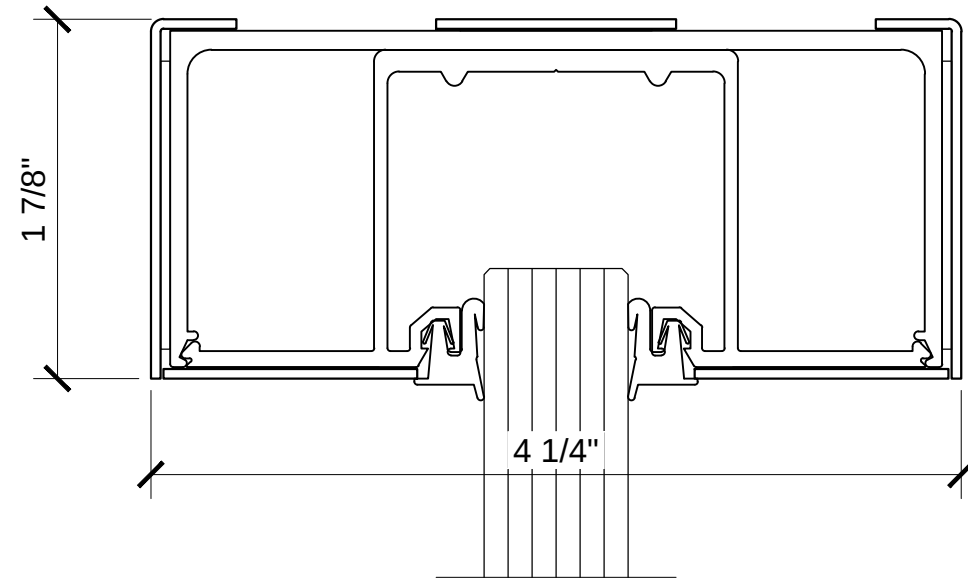
1 3/4" x 4" CLAD HEADER W/ GLAZING POCKET DCH4 SERIES
