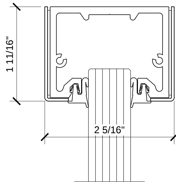
1 11/16" x 2 5/16" CLAD HEADER W/ GLAZING POCKET NH3 SERIES
