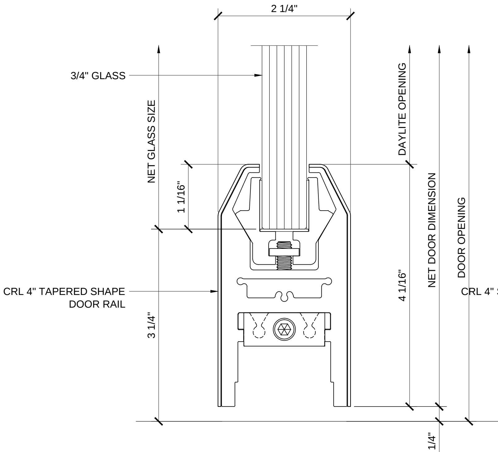
CRL DR4T34 4" TALL TAPERED DOOR RAIL
