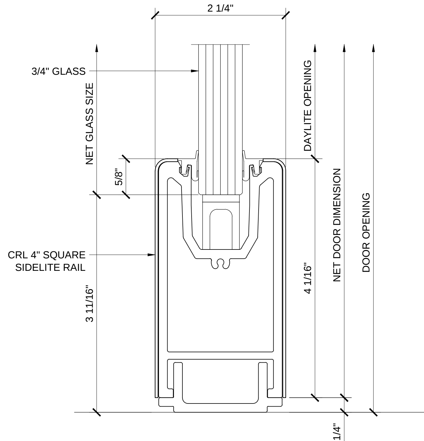
CRL 4" TALL SQUARE SIDELITE RAIL
