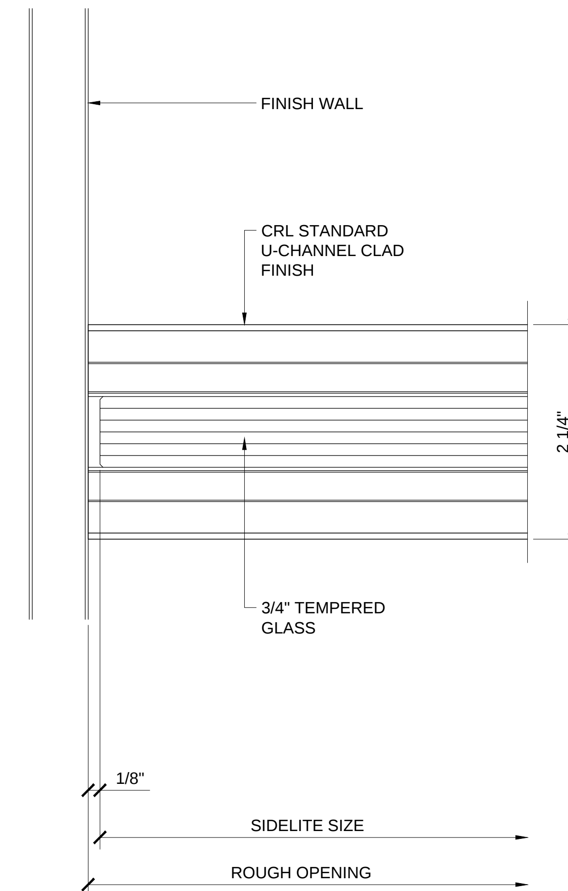
PLAN VIEW @ JAMB
