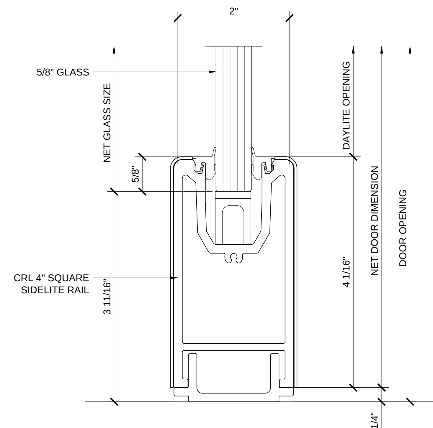
CRL 4" TALL SQUARE SIDELITE RAIL
