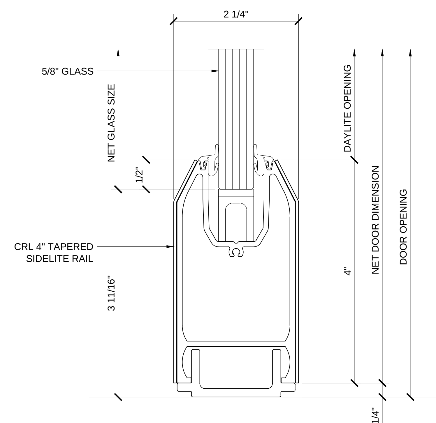
CRL 4" TALL TAPERED SIDELITE RAIL
