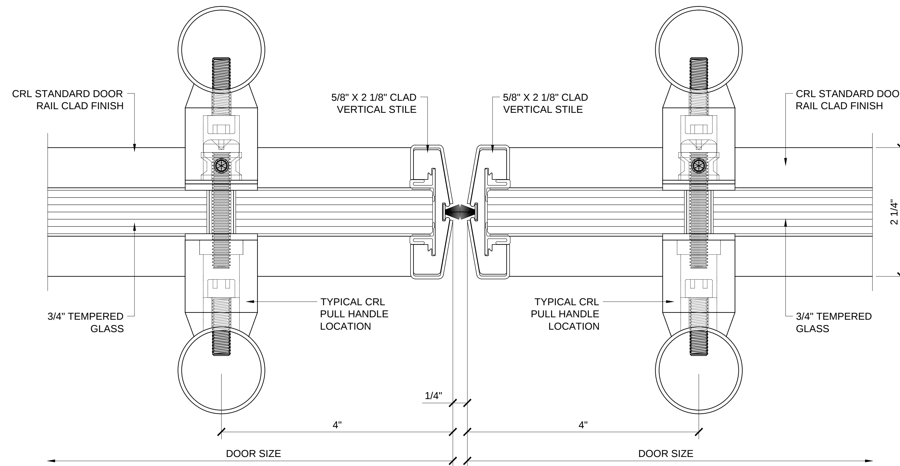
PLAN VIEW @ MEETING SECTION
