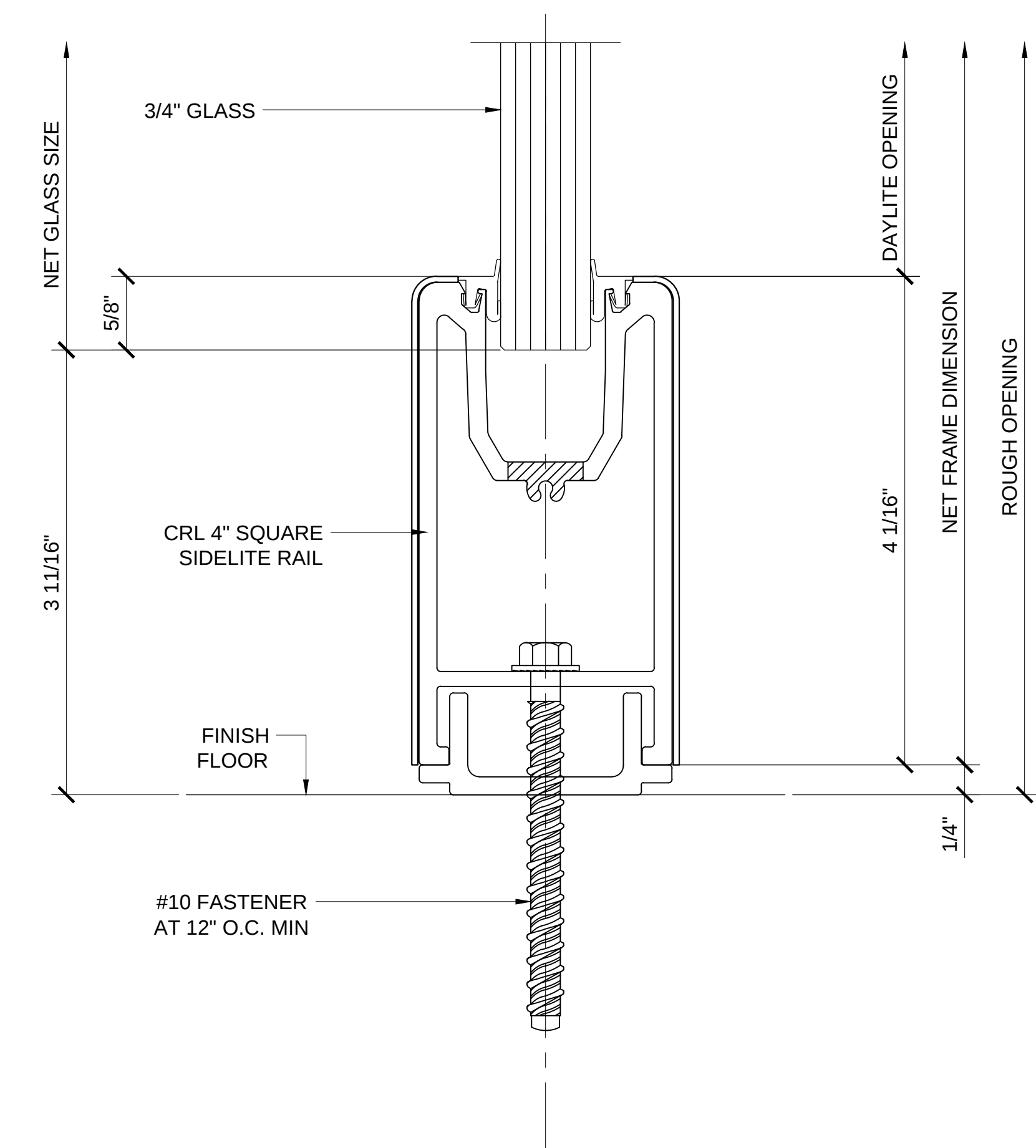
SECTION DETAIL @ SILL (MATCHES DOOR) (2.4)
