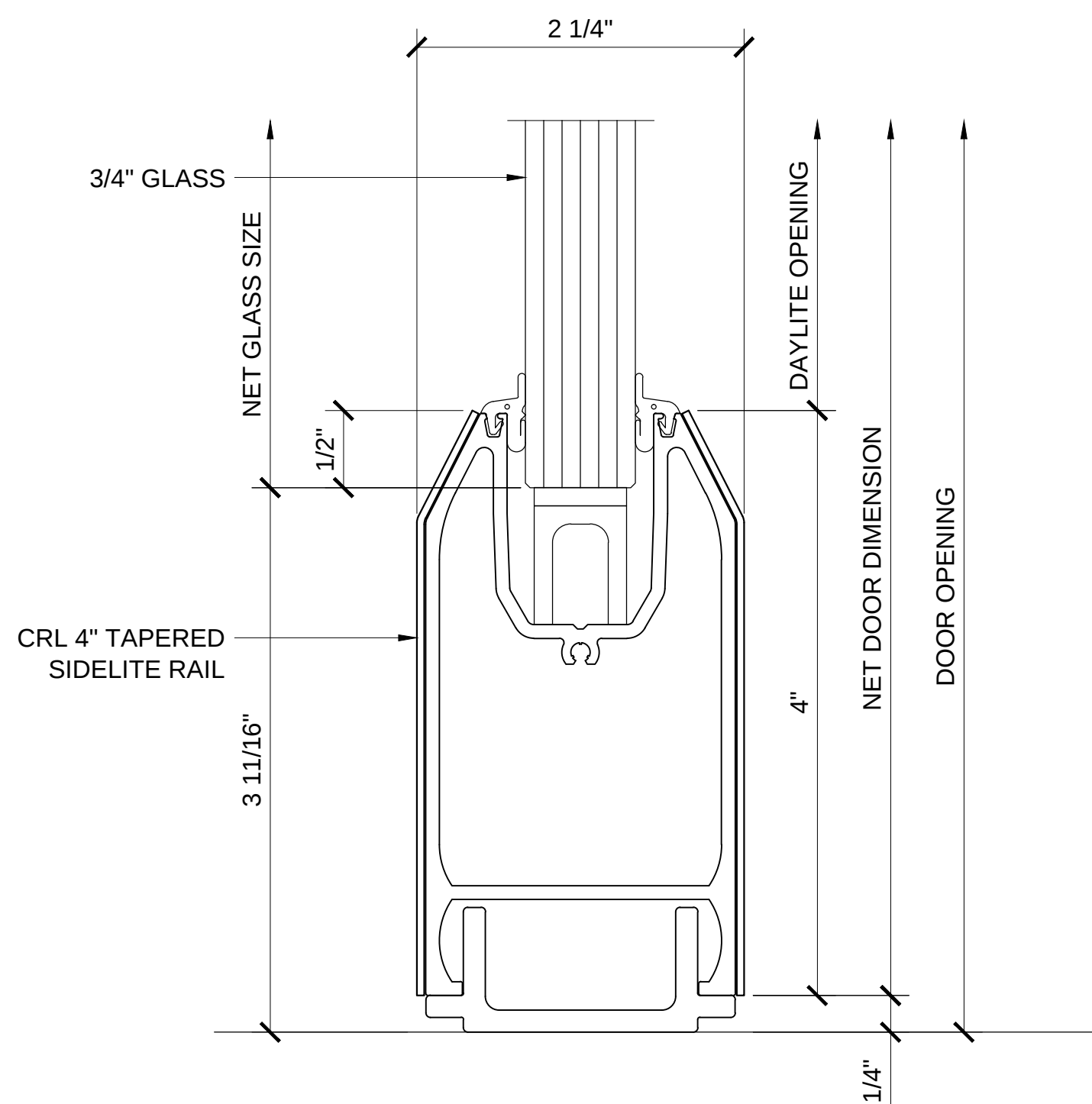
CRL 4" TALL TAPERED SIDELITE RAIL
