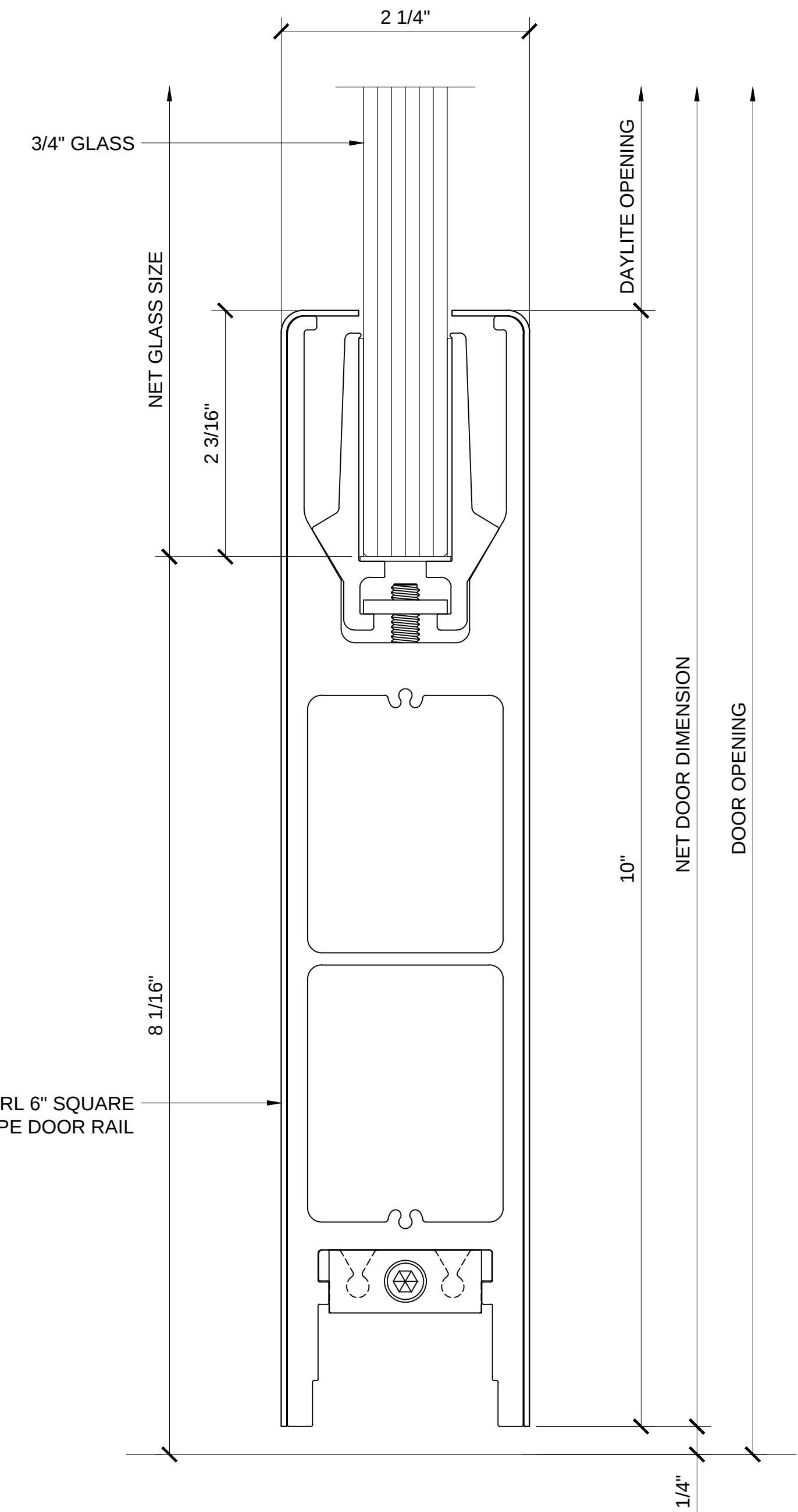
CRL DR10S34 10" TALL SQUARE DOOR RAIL
