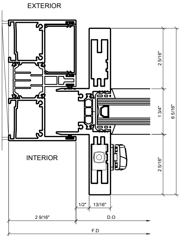
① STRIKE JAMB AT SLIDER 1'-0"=1'-0" ARCH REF: N/A
