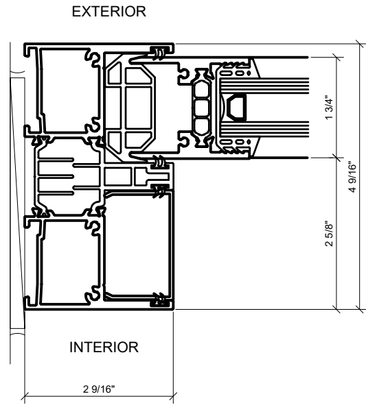
1 WALL JAMB AT FIXED PANEL 1'-0"=1'-0" ARCH REF: N/A
