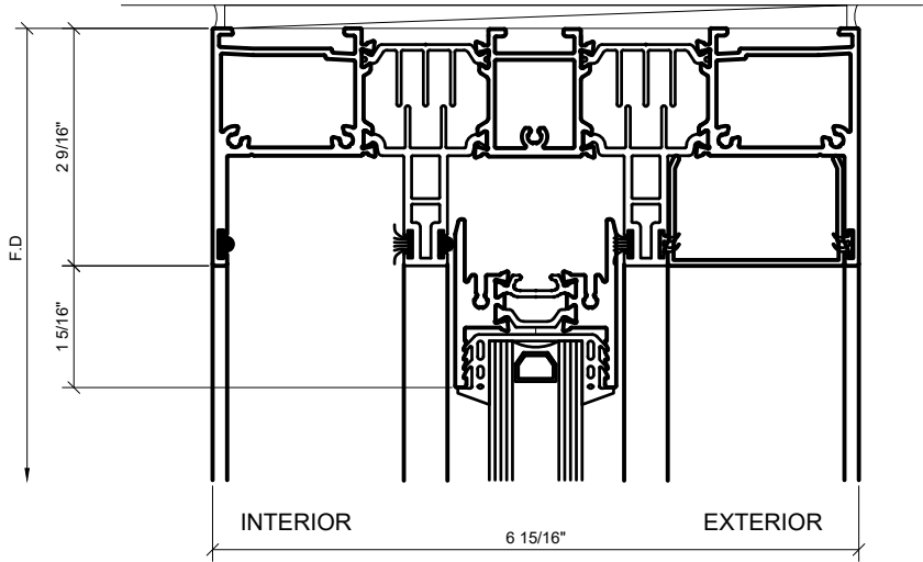
⑤ HEAD AT FIXED PANEL 5 ARCH REF: N/A
