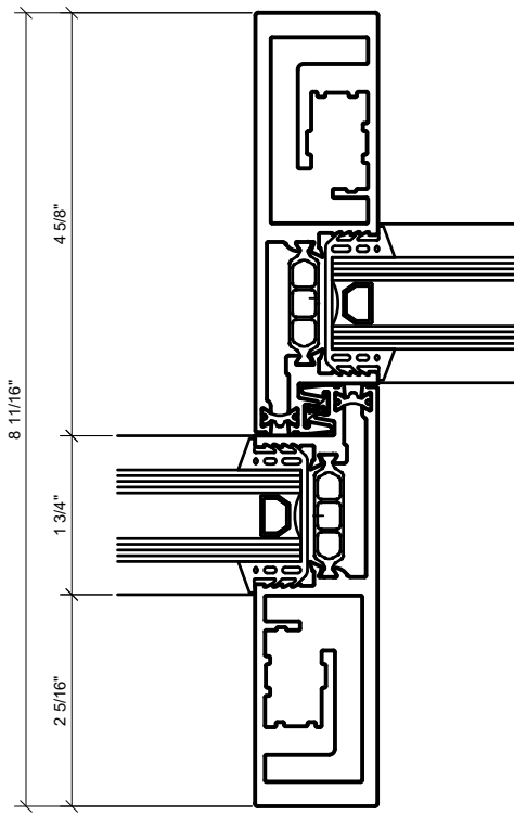
6 INTERLOCKER VERTICAL ( EXTERIOR ) 1'-0"=1'-0" ARCH REF: N/A
