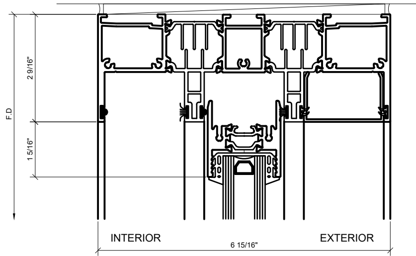
③ HEAD AT SLIDER OPENING 1'-0"=1'-0" ARCH REF: N/A
