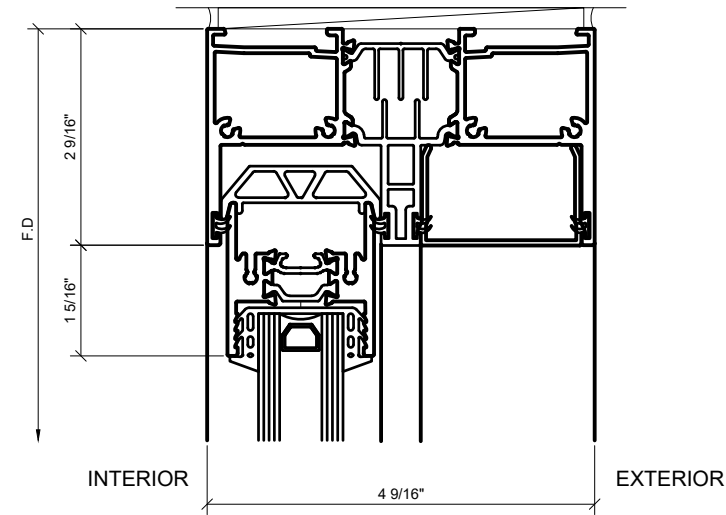
5 HEAD AT FIXED PANEL 1'-0"=1'-0" ARCH REF: N/A
