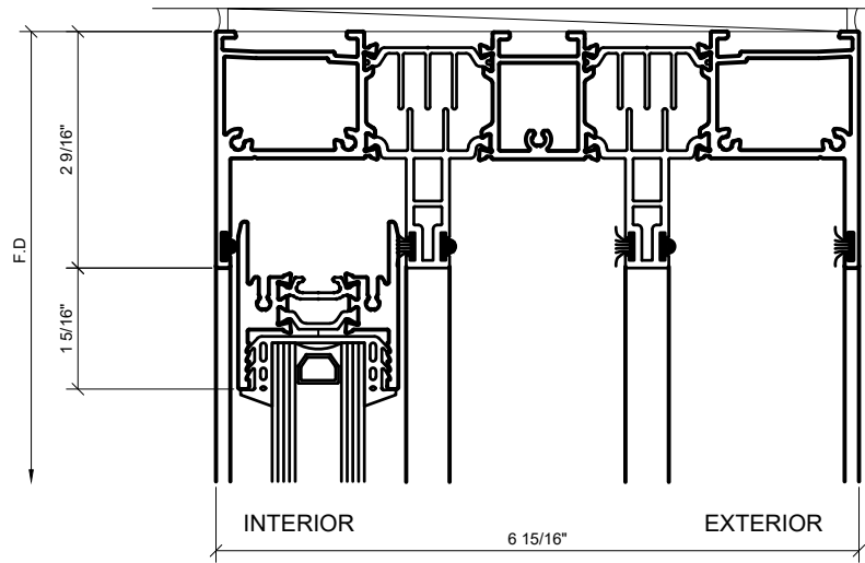
① HEAD AT SLIDER OPENING 1'-0"=1'-0" ARCH REF: N/A
