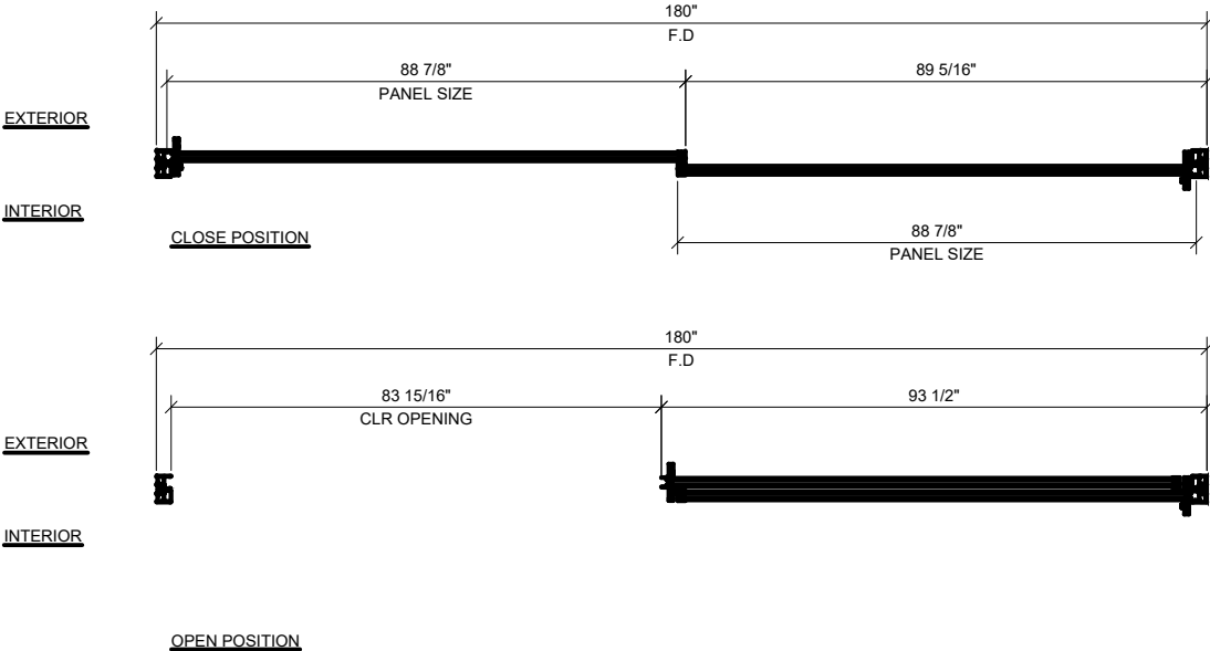
1 XX - 2 TRACK CONFIGURATION 3/4" = 1'-0" ARCH. REF.: N/A
