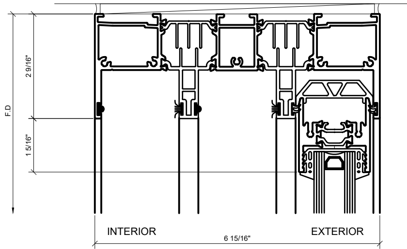
① HEAD AT FIXED PANEL 1'-0"=1'-0" ARCH REF: N/A
