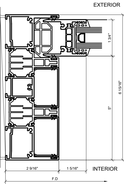
① WALL JAMB AT FIXED PANEL 1'-0"=1'-0" ARCH REF: N/A
