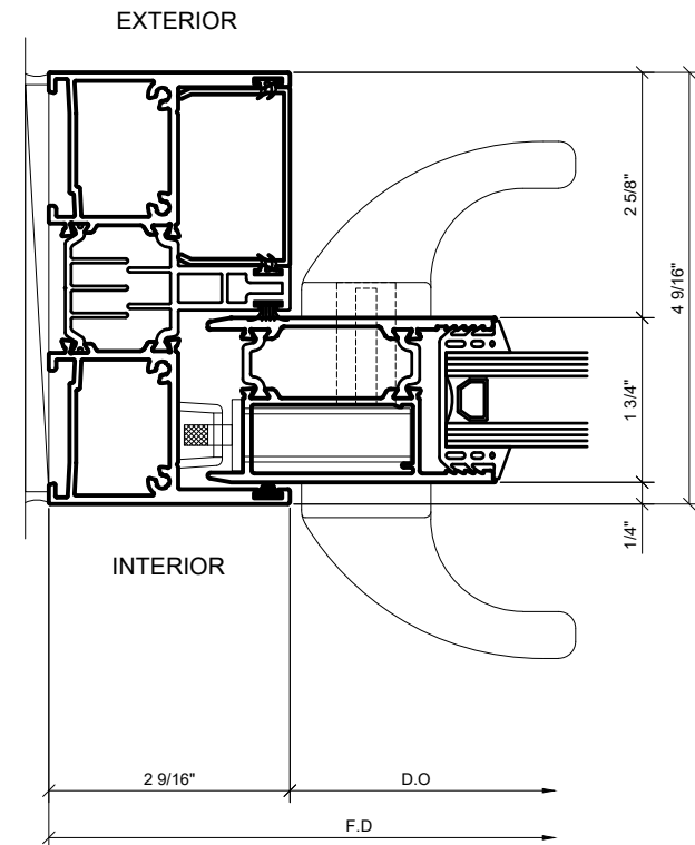
①A STRIKE JAMB W/HOOK LOCK (OPTIONAL) 1'-0"=1'-0" ARCH REF: N/A
