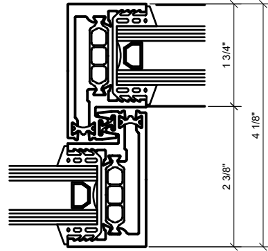
② INETERLOCKER VERTICAL ( INTERIOR ) 1'-0"=1'-0" ARCH REF: N/A
