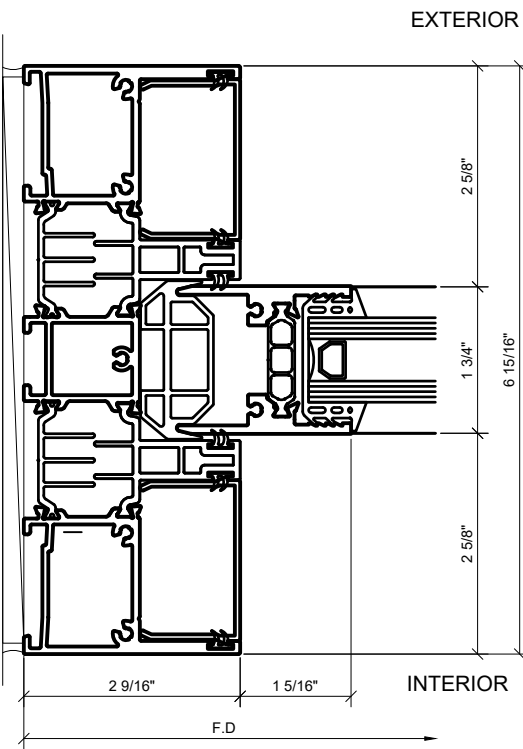
② INETERLOCKER VERTICAL ( INTERIOR ) 1'-0"=1'-0" ARCH REF: N/A
