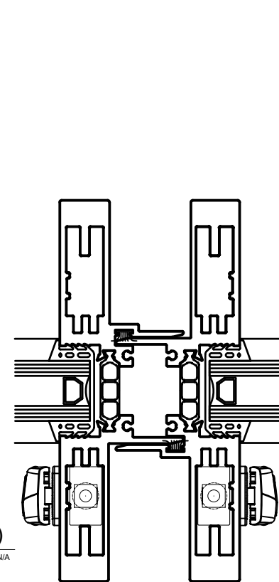
③ MEETING VERTICAL 1'-0"=1'-0" ARCH REF: N/A
