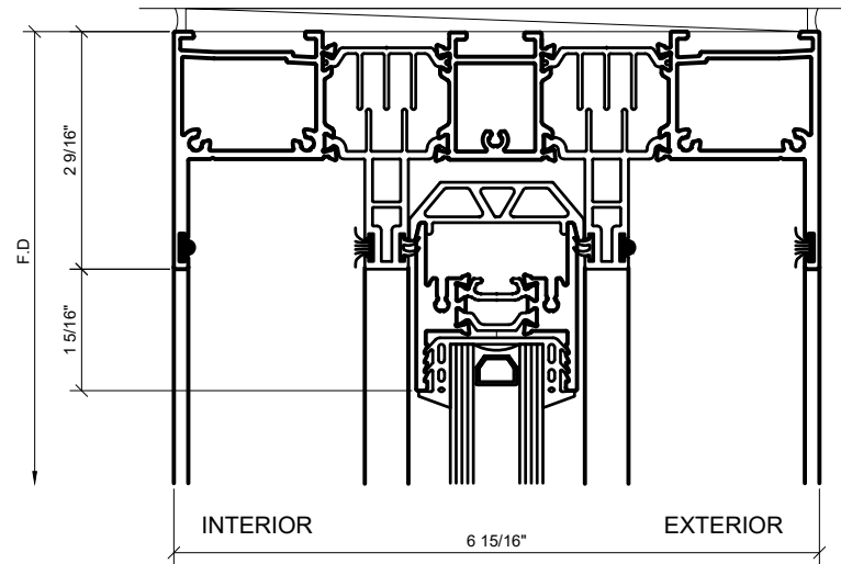
③ HEAD AT FIXED PANEL 1'-0"=1'-0" ARCH REF: N/A
