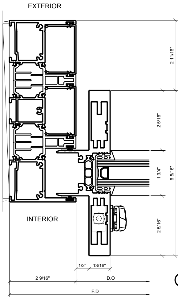
② INETERLOCKER VERTICAL ( INTERIOR ) 1'-0"=1'-0" ARCH REF: N/A
