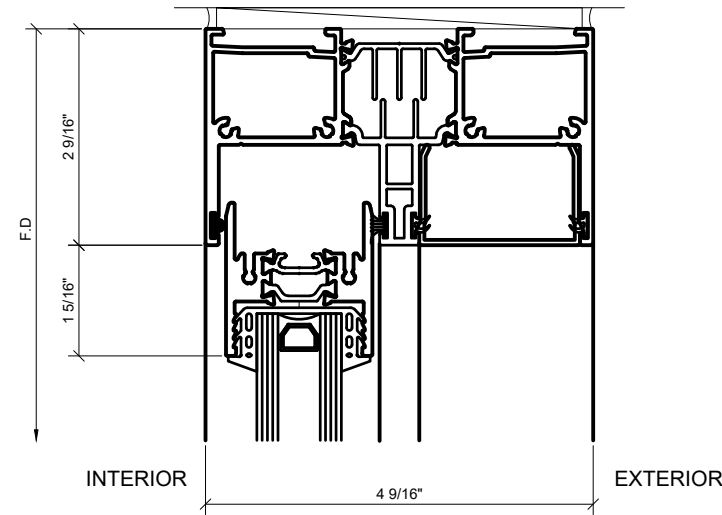
1 HEAD AT SLIDER OPENING 1'-0"=1'-0" ARCH REF: N/A
