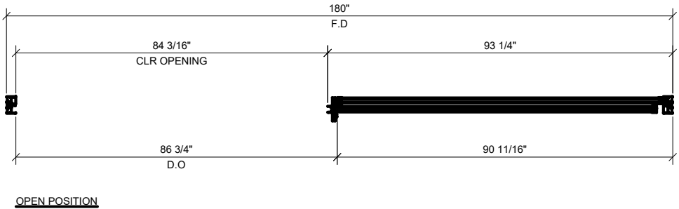
① XO - 2 TRACK CONFIGURATION 3/4" = 1'-0" ARCH. REF.: N/A
