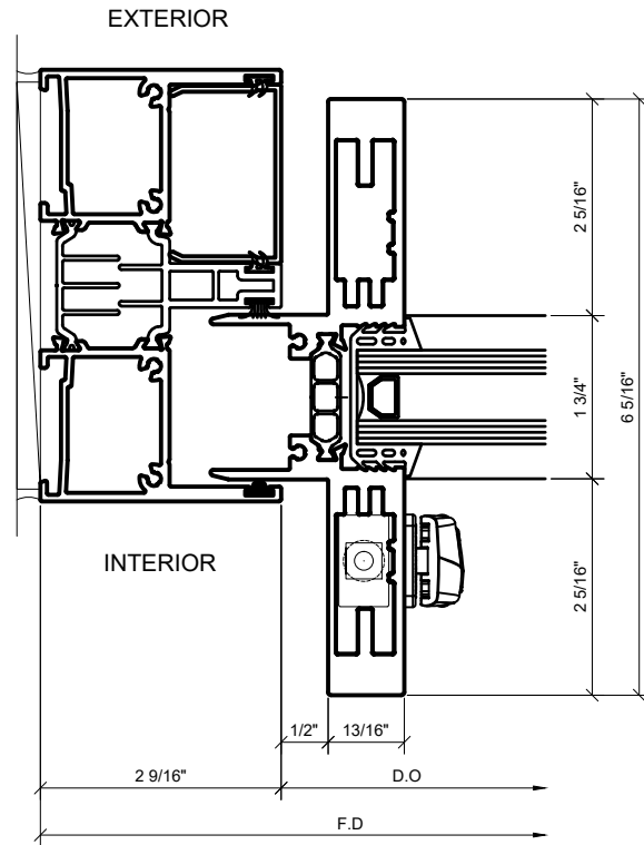
① STRIKE JAMB AT SLIDER 1'-0"=1'-0" ARCH REF: N/A
