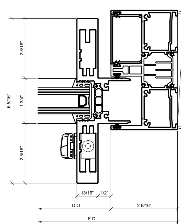
④ STRIKE JAMB AT SLIDER 1'-0"=1'-0" ARCH REF: N/A
