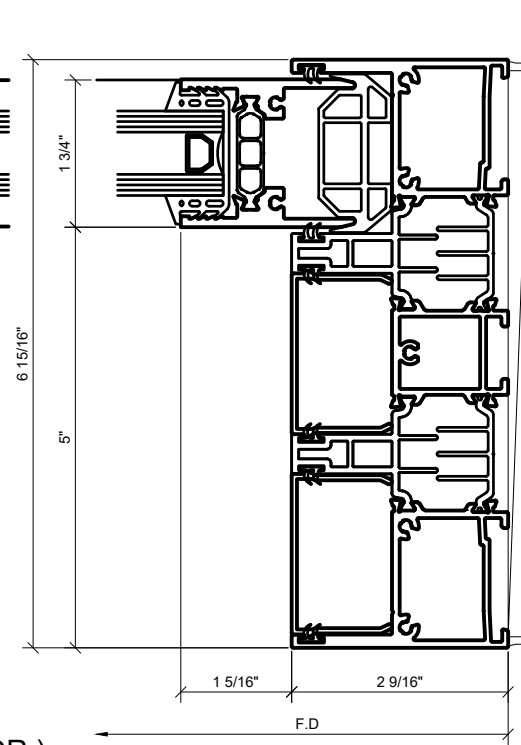
⑤ WALL JAMB AT FIXED PANEL 1'-0"=1'-0" ARCH REF: N/A
