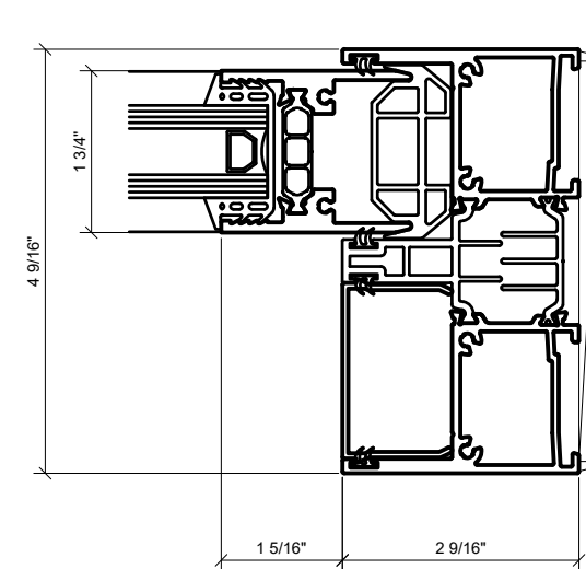
④ WALL JAMB AT FIXED PANEL 1'-0"=1'-0" ARCH REF: N/A
