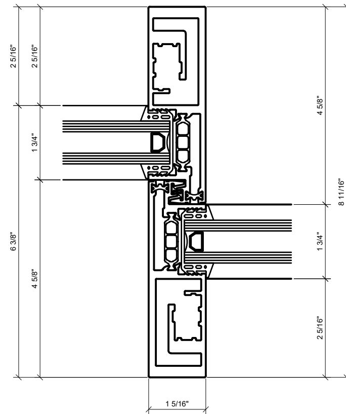
④ INTERLOCKER VERTICAL ( EXTERIOR ) 1'-0"=1'-0" ARCH REF: N/A
