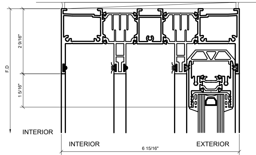
⑤ HEAD AT FIXED PANEL 1'-0"=1'-0" ARCH REF: N/A
