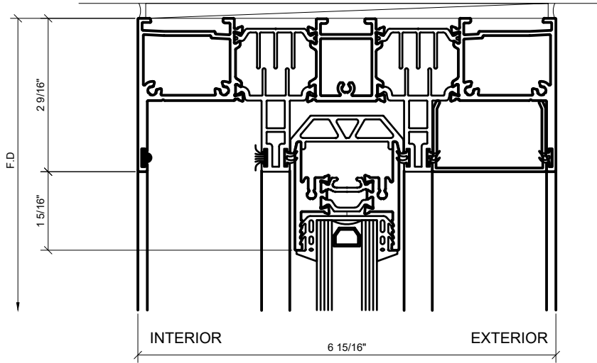
① HEAD AT SLIDER OPENING 1'-0"=1'-0" ARCH REF: N/A
