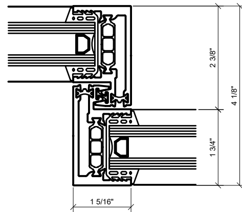
③ INETERLOCKER VERTICAL ( INTERIOR ) 1'-0"=1'-0" ARCH REF: N/A
