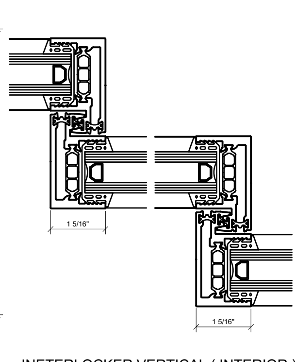
② INETERLOCKER VERTICAL ( INTERIOR ) 1'-0"=1'-0" ARCH REF: N/A
