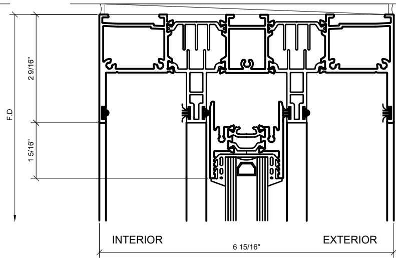
③ HEAD AT SLIDER OPENING 1'-0"=1'-0" ARCH REF: N/A
