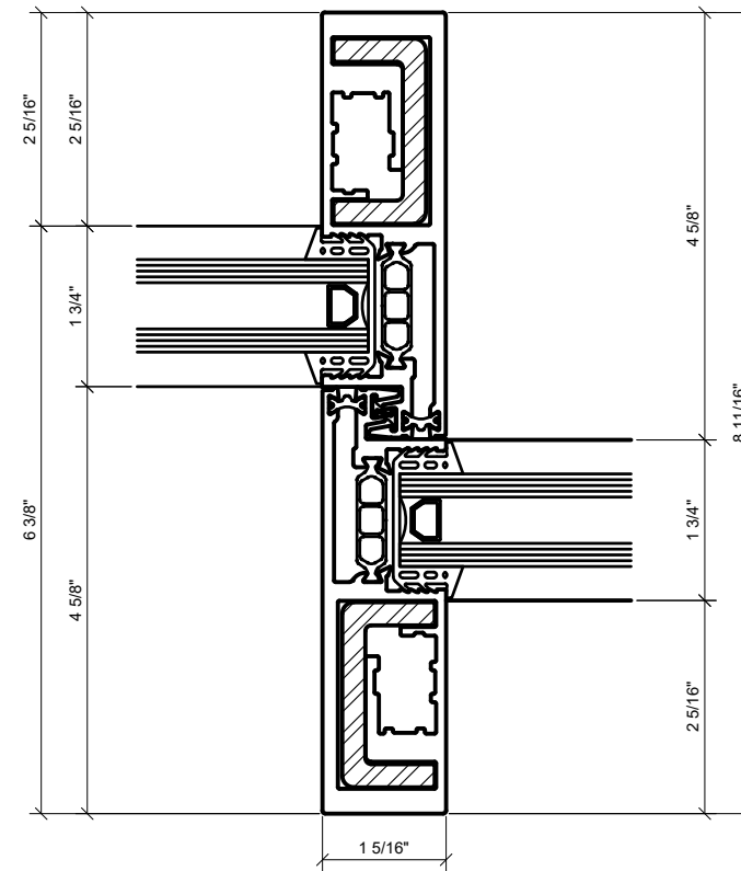
③ STRIKE JAMB AT SLIDER 1'-0"=1'-0" ARCH REF: N/A
