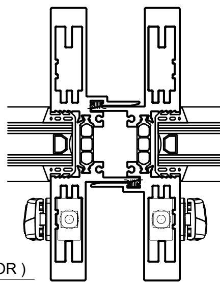
③ MEETING VERTICAL 1'-0"=1'-0" ARCH REF: N/A
