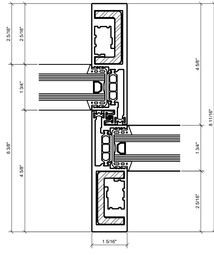
⑤ INTERLOCKER VERTICAL W/REINFORCEMENT 1'-0"=1'-0" ARCH REF: N/A
