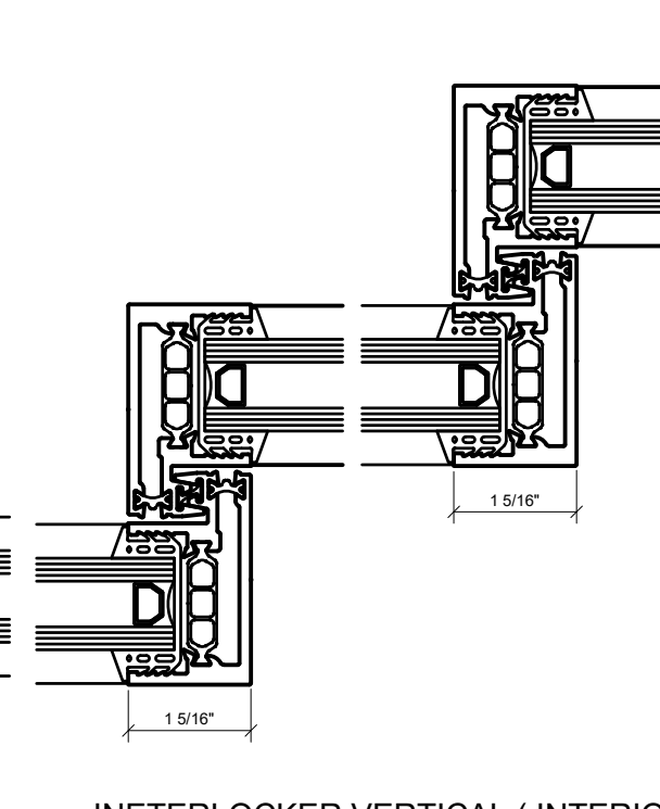
④ INETERLOCKER VERTICAL ( INTERIOR ) 1'-0"=1'-0" ARCH REF: N/A
