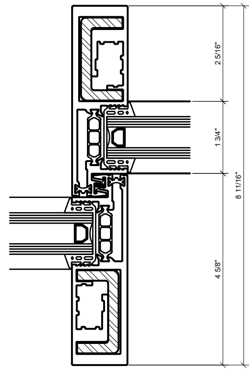
7 INTERLOCKER VERTICAL W/REINFORCEMENT 1'-0"=1'-0" ARCH REF: N/A
