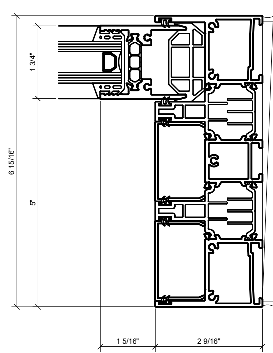
③ INETERLOCKER VERTICAL ( INTERIOR ) 1'-0"=1'-0" ARCH REF: N/A
