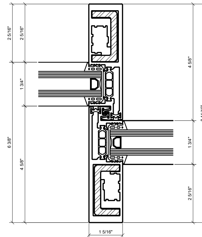
⑤ INTERLOCKER VERTICAL W/REINFORCEMENT 1'-0"=1'-0" ARCH REF: N/A
