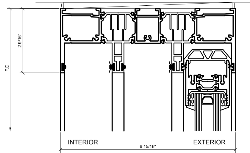
⑤ HEAD AT SLIDER OPENING 1'-0"=1'-0" ARCH REF: N/A
