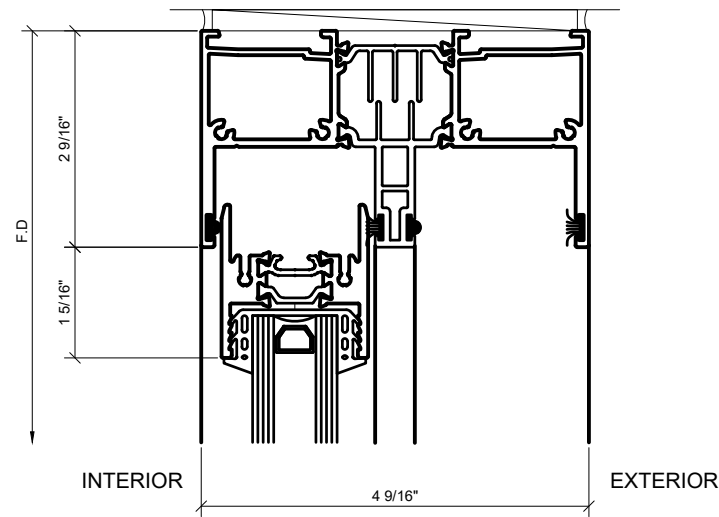
③ HEAD AT SLIDER OPENING 1'-0"=1'-0" ARCH REF: N/A
