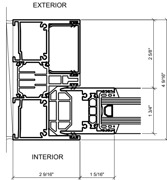
① WALL JAMB AT FIXED PANEL 1'-0"=1'-0" ARCH REF: N/A
