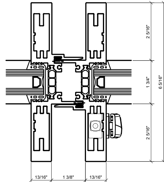
② MEETING VERTICAL 1'-0"=1'-0" ARCH REF: N/A
