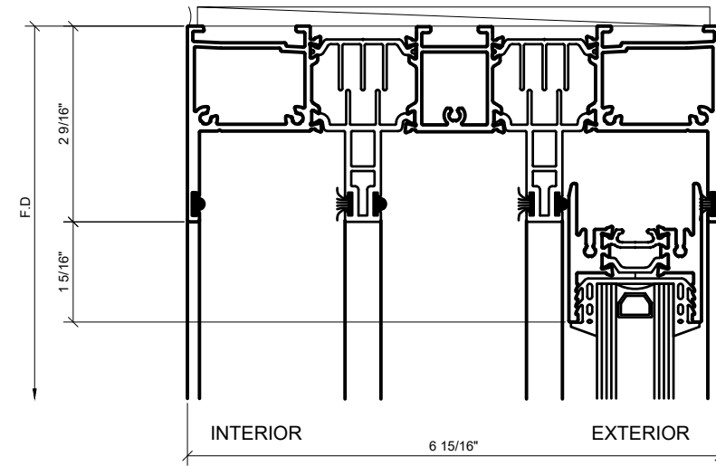
⑤ HEAD AT SLIDER OPENING 1'-0"=1'-0" ARCH REF: N/A
