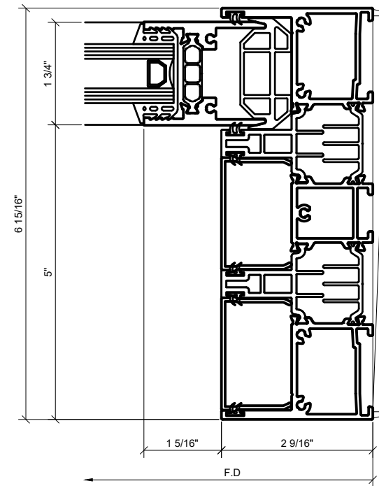
⑤ WALL JAMB AT FIXED PANEL 1'-0"=1'-0" ARCH REF: N/A
