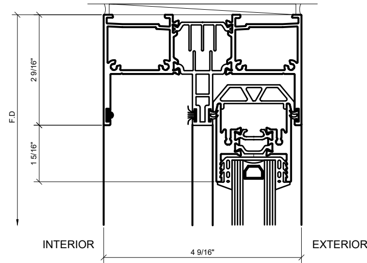
3 HEAD AT FIXED PANEL 1'-0"=1'-0" ARCH REF: N/A
