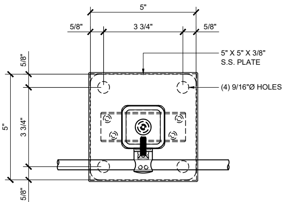
CBR STANDOFF CONNECTOR (FLAT BACK / FLANGE)
