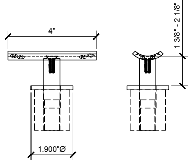
P7VF W/ PRS1 SADDLE
