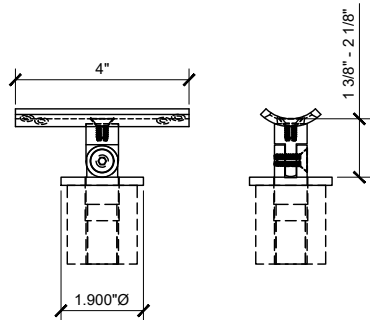
P7VS W/ PRS1 SADDLE
