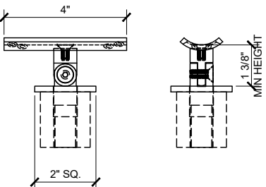
P1VS W/ PRS1 SADDLE
