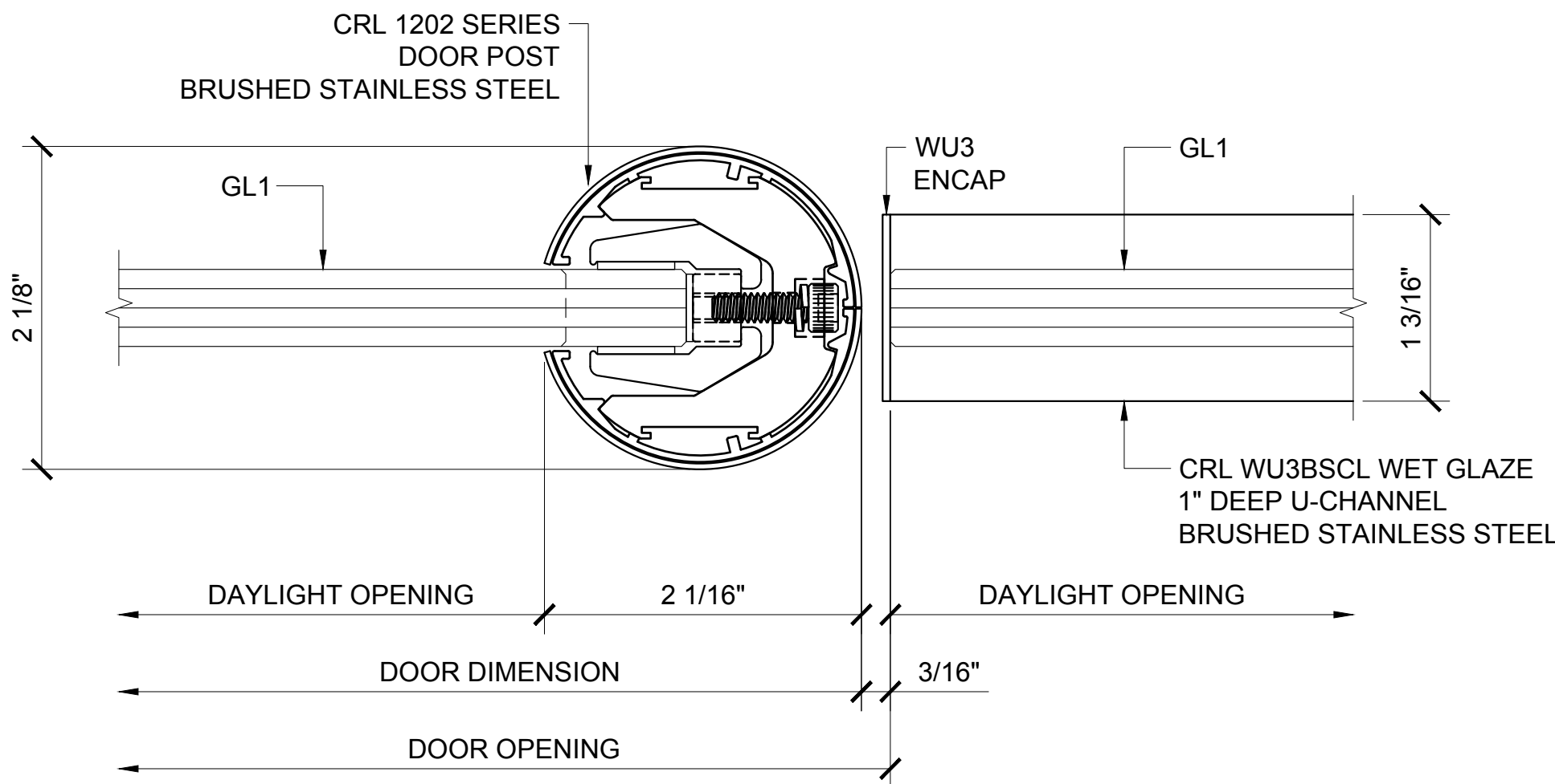
② DOOR PIVOT POST SECTION DETAIL
