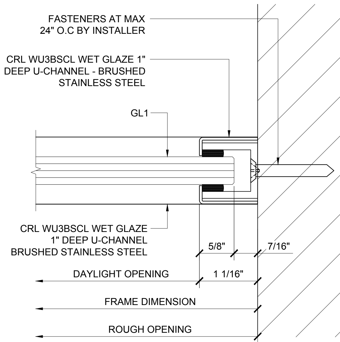
③ WALL JAMB DETAIL
