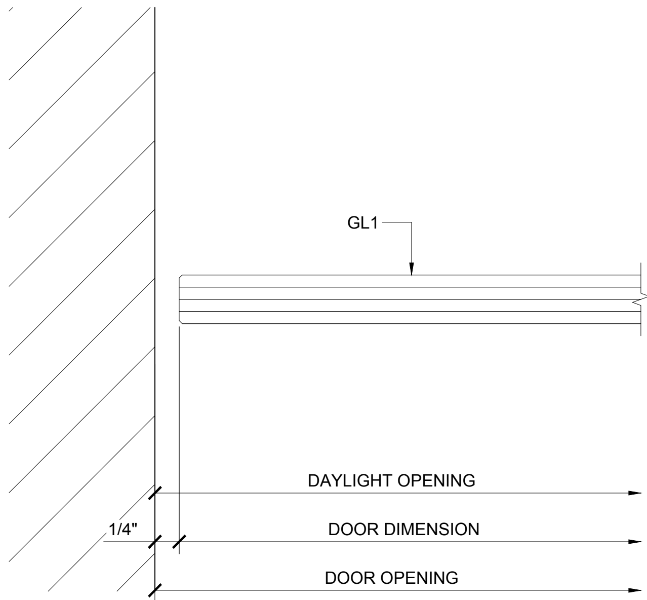
① DOOR JAMB AT WALL
