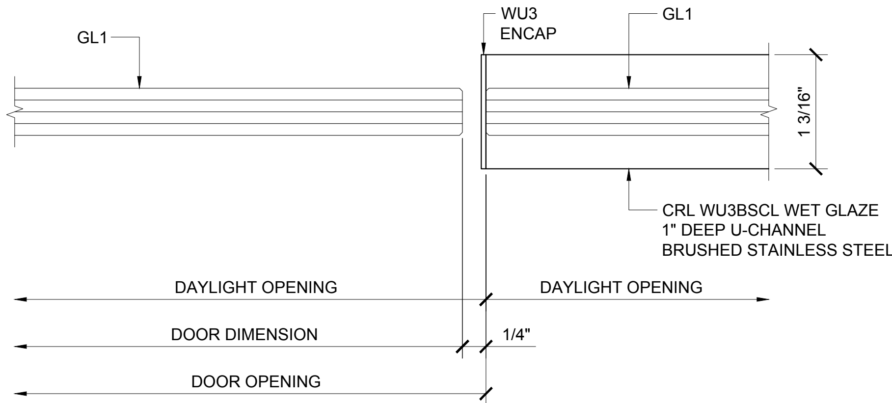
② DOOR JAMB AT SIDELITE
