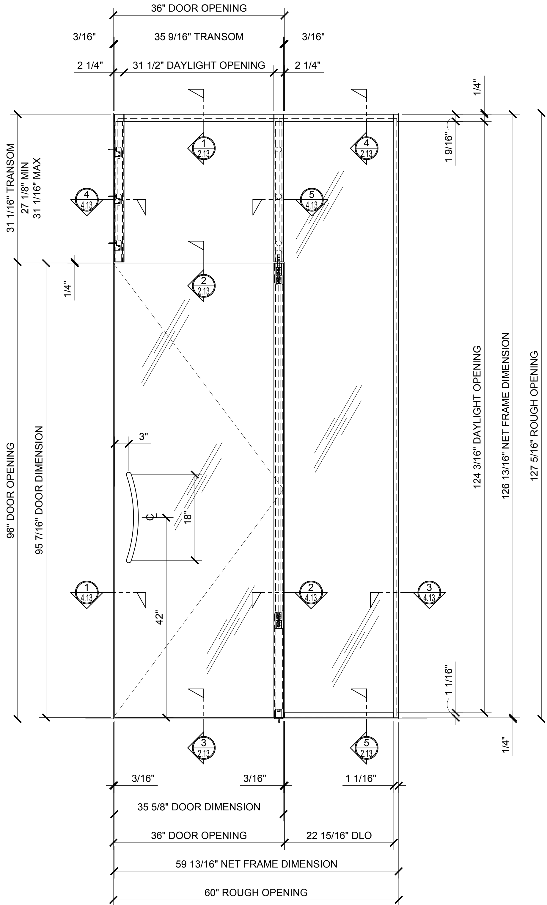
4 ELEVATION ARCH REF: 1"=1'-0"
