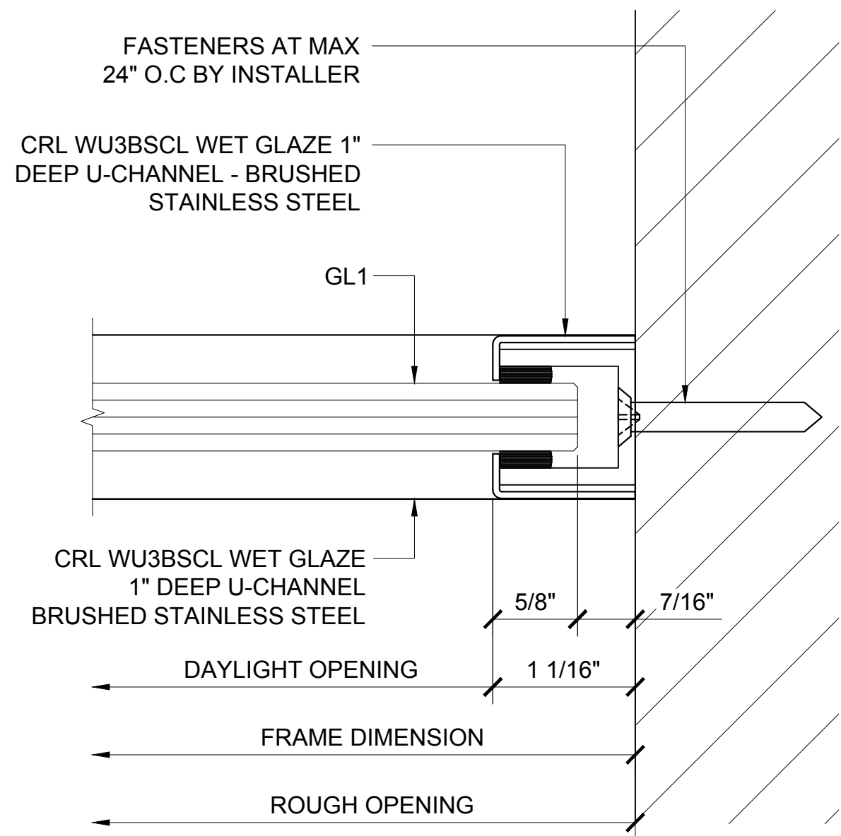
③ WALL JAMB DETAIL
