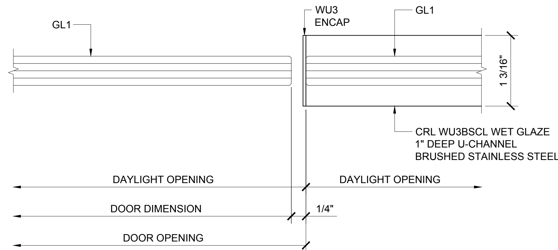
② DOOR JAMB AT SIDELITE ARCH REF: 1'-0"=1'-0"
