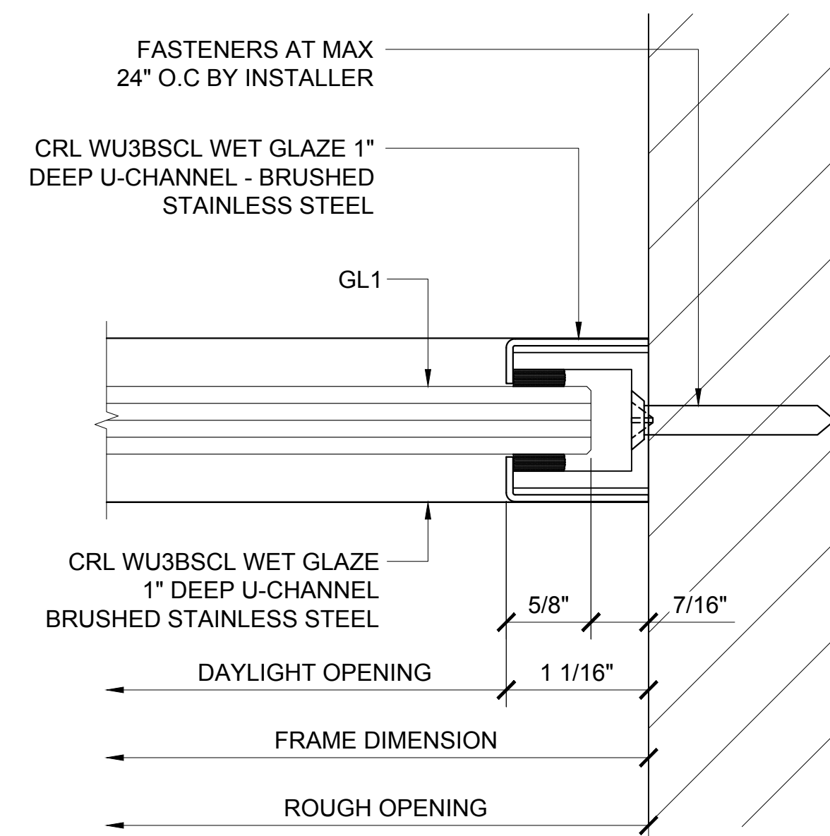
③ WALL JAMB DETAIL ARCH REF: 1'-0"=1'-0"
