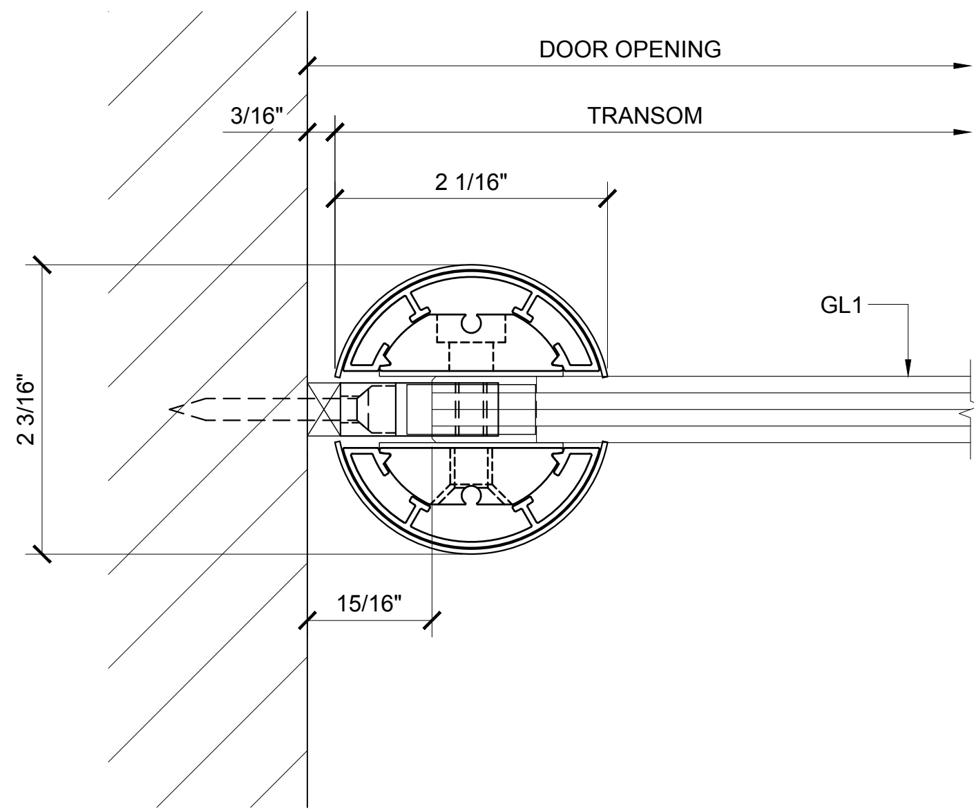
④ TRANSOM POST SECTION AT WALL DETAIL ARCH REF: 1'-0"=1'-0"
