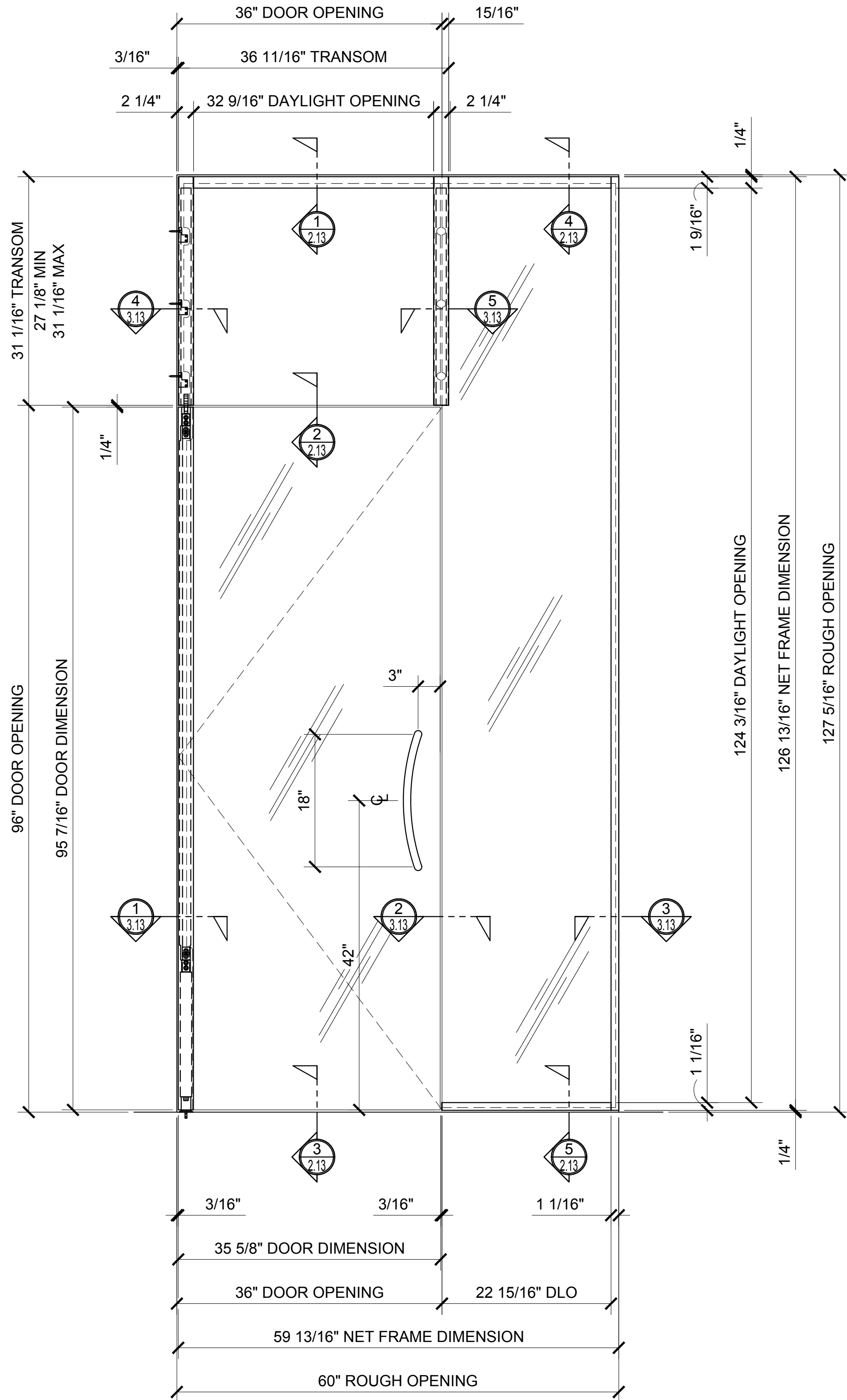
2 ELEVATION ARCH REF: 1"=1'-0"
