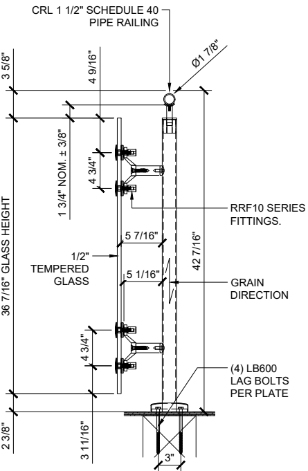
WOOD MOUNT 1 1/2"=1'-0"
