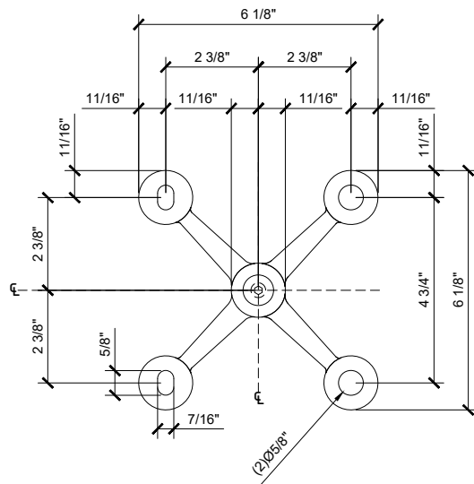
GRP4 SERIES SPIDER FITTING 6"=1'-0"
