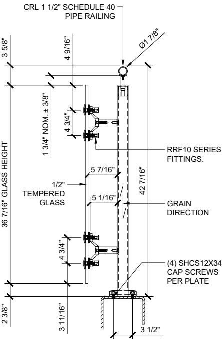
STEEL MOUNT 1 1/2"=1'-0"
