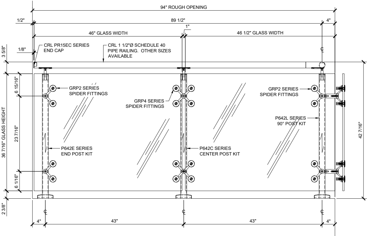
TYPICAL ELEVATION 1 1/2"=1'-0"
