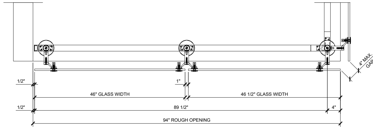
TYPICAL PLAN VIEW 1 1/2"=1'-0"
