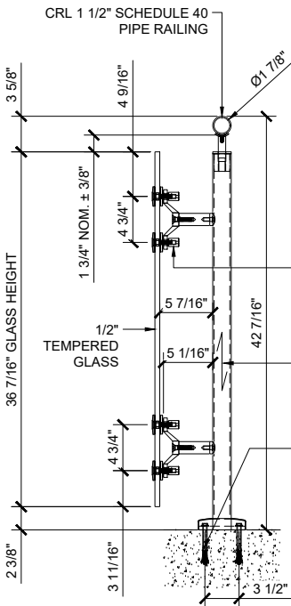
CONCRETE MOUNT 1 1/2"=1'-0"
