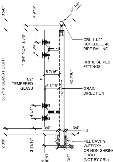
CORE MOUNT 1 1/2"=1'-0"
