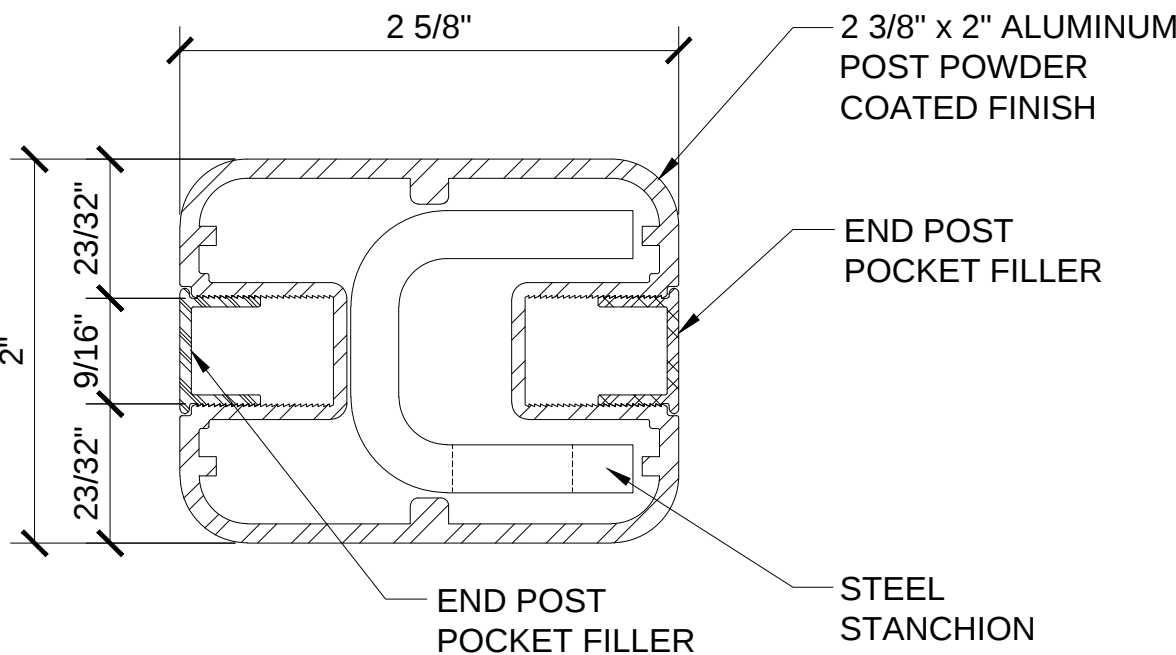
CRL AWS 2" x 2 5/8" RECTANGULAR 180° ALUMINUM GATE POST *
