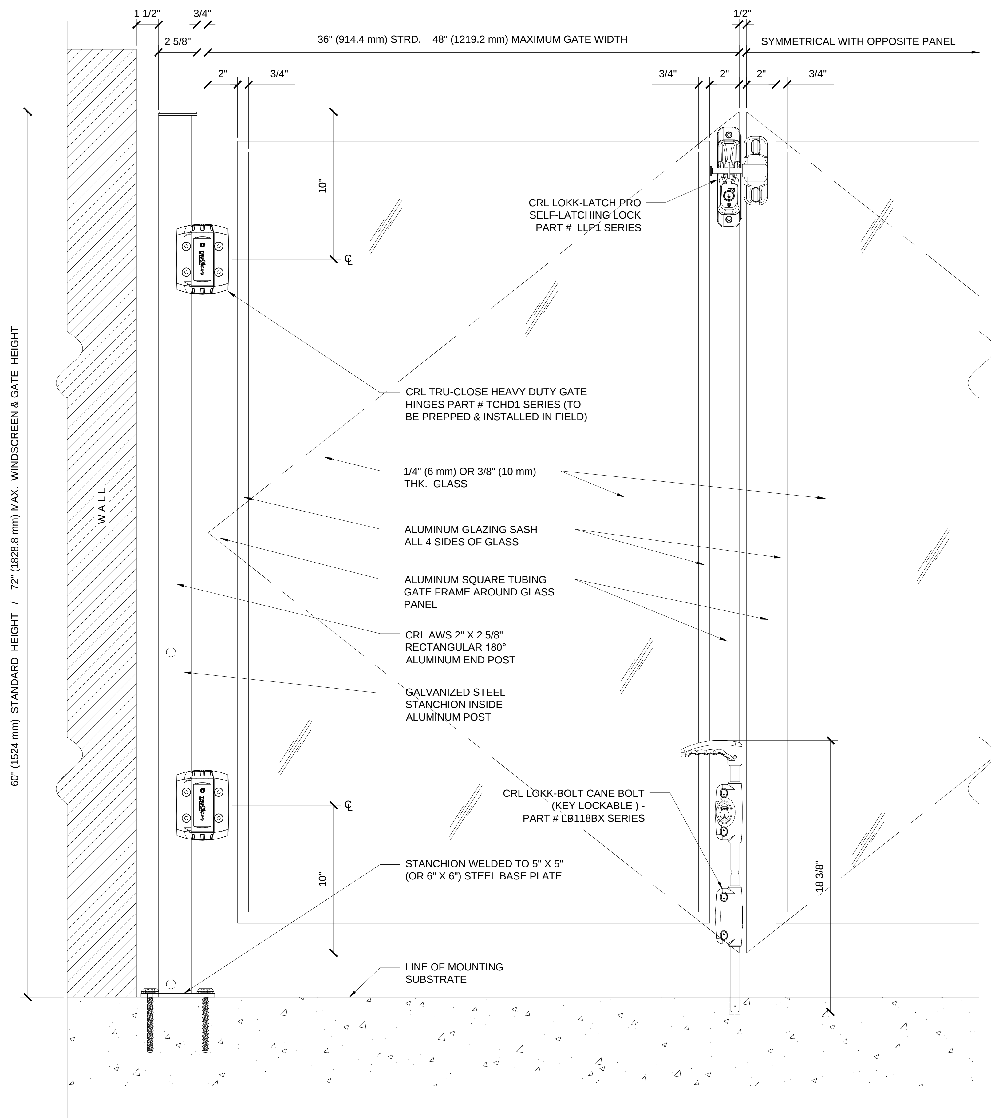
2 WINDSCREEN PAIR GATE ELEVATION
