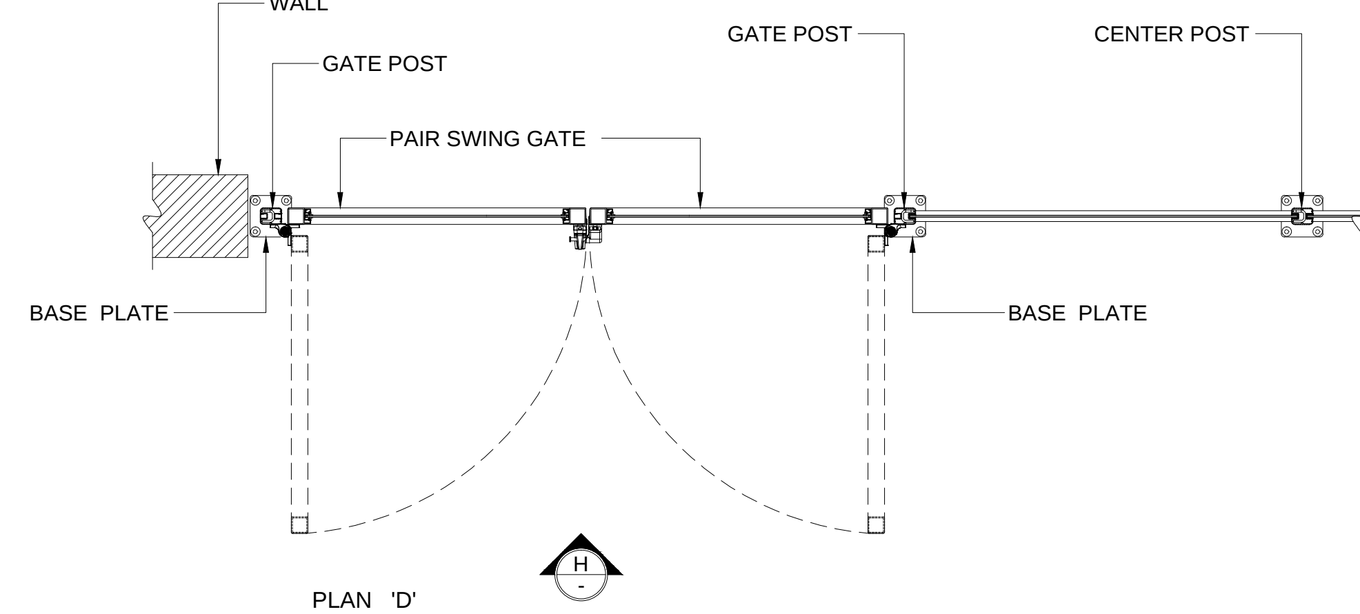
2 WINDSCREEN (w/ PAIR SWING GATES ADJACENT TO WALL) WITH SURFACE MOUNT STANCHIONS SCALE: 3/4"=1'-0"
