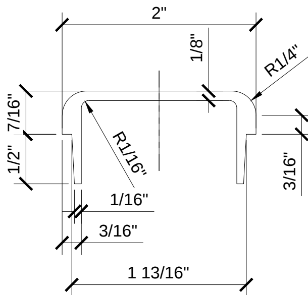
CAP SECTION A-A
