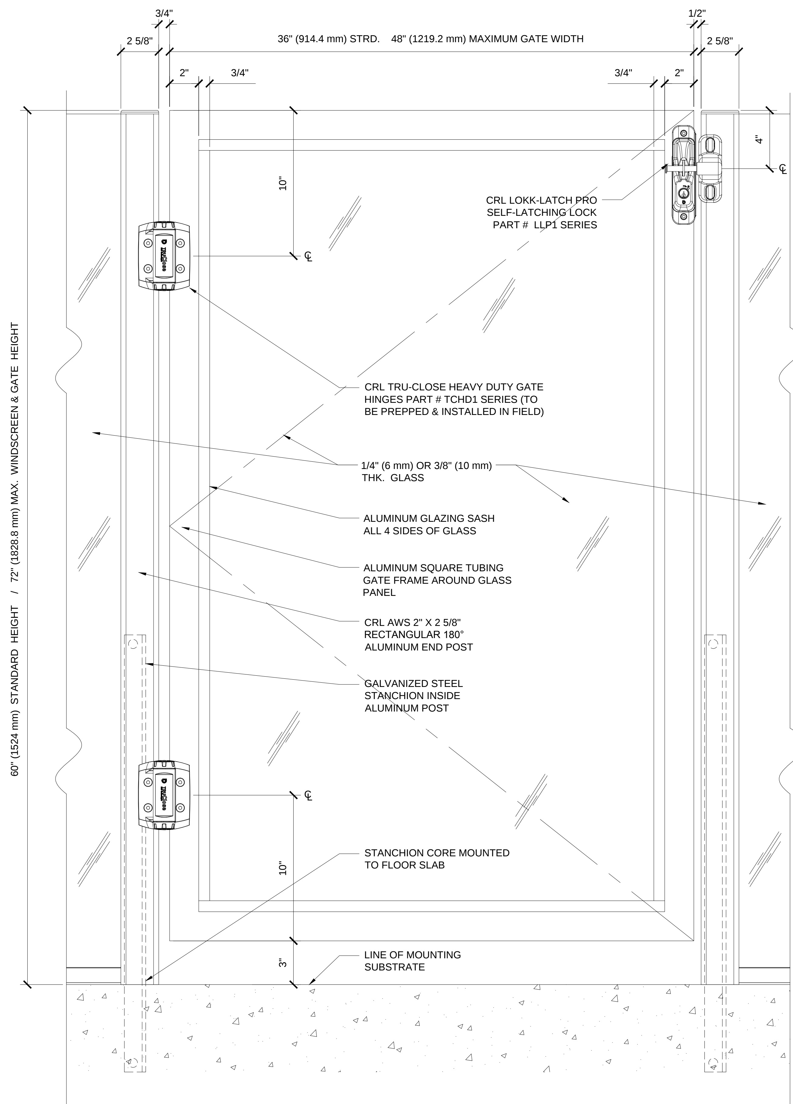
1 WINDSCREEN SINGLE GATE ELEVATION
