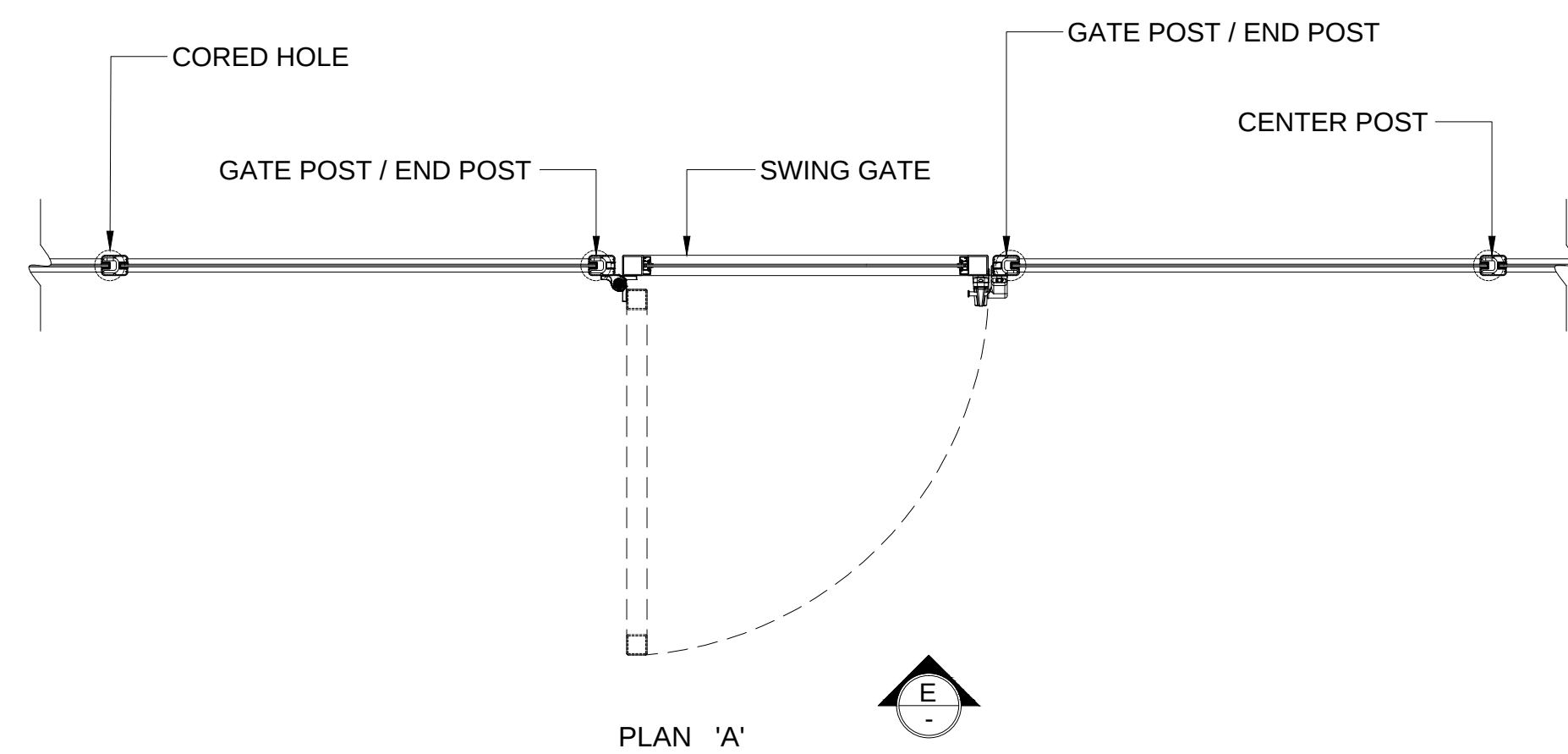
1 TYPICAL ALUMINUM WINDSCREEN - (w/ SINGLE SWING GATE) WITH STANCHIONS THRU CORE DRILLED HOLES SCALE: 3/4"=1'-0"
