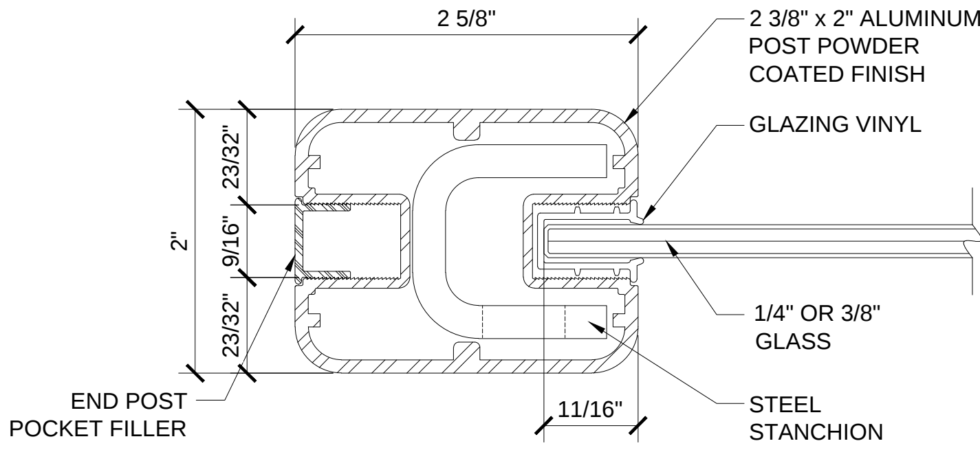
CRL AWS 2" x 2 5/8" RECTANGULAR 180° ALUMINUM GATE POST / END POST *
