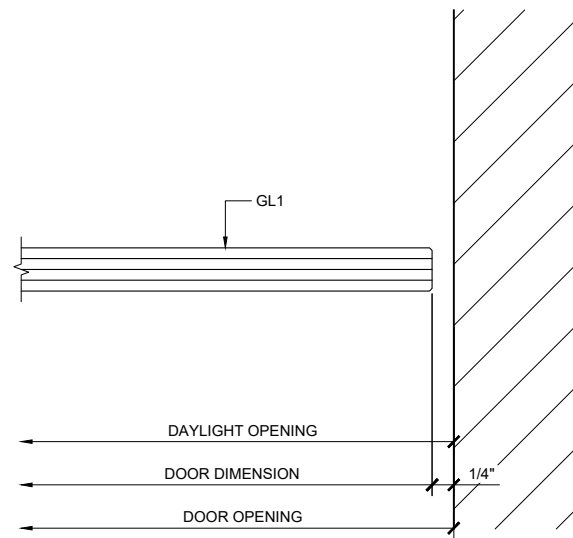
③ DOOR JAMB AT WALL ARCH REF: 1'-0"=1'-0"
