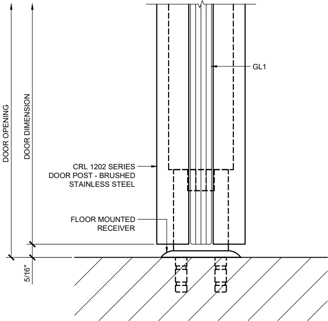
② DOOR SILL DETAIL ARCH REF: 1'-0"=1'-0"
