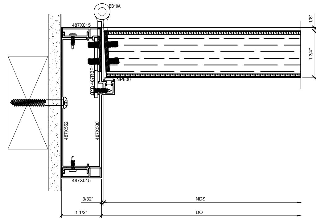
③ SURFACE MOUNT DOOR JAMB DETAIL AT HINGE SIDE WITH WOOD FLUSH DOOR ARCH REF: 1'-0"=1'-0"
