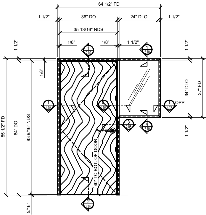
② ELEVATION: WOOD DOOR WITH ABOVE FLOOR SIDELITE ARCH REF: NONE 3/4"=1'-0"
