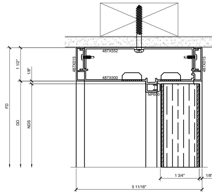
③ SURFACE MOUNTED DOOR HEAD DETAIL WITH WOOD FLUSH DOOR
