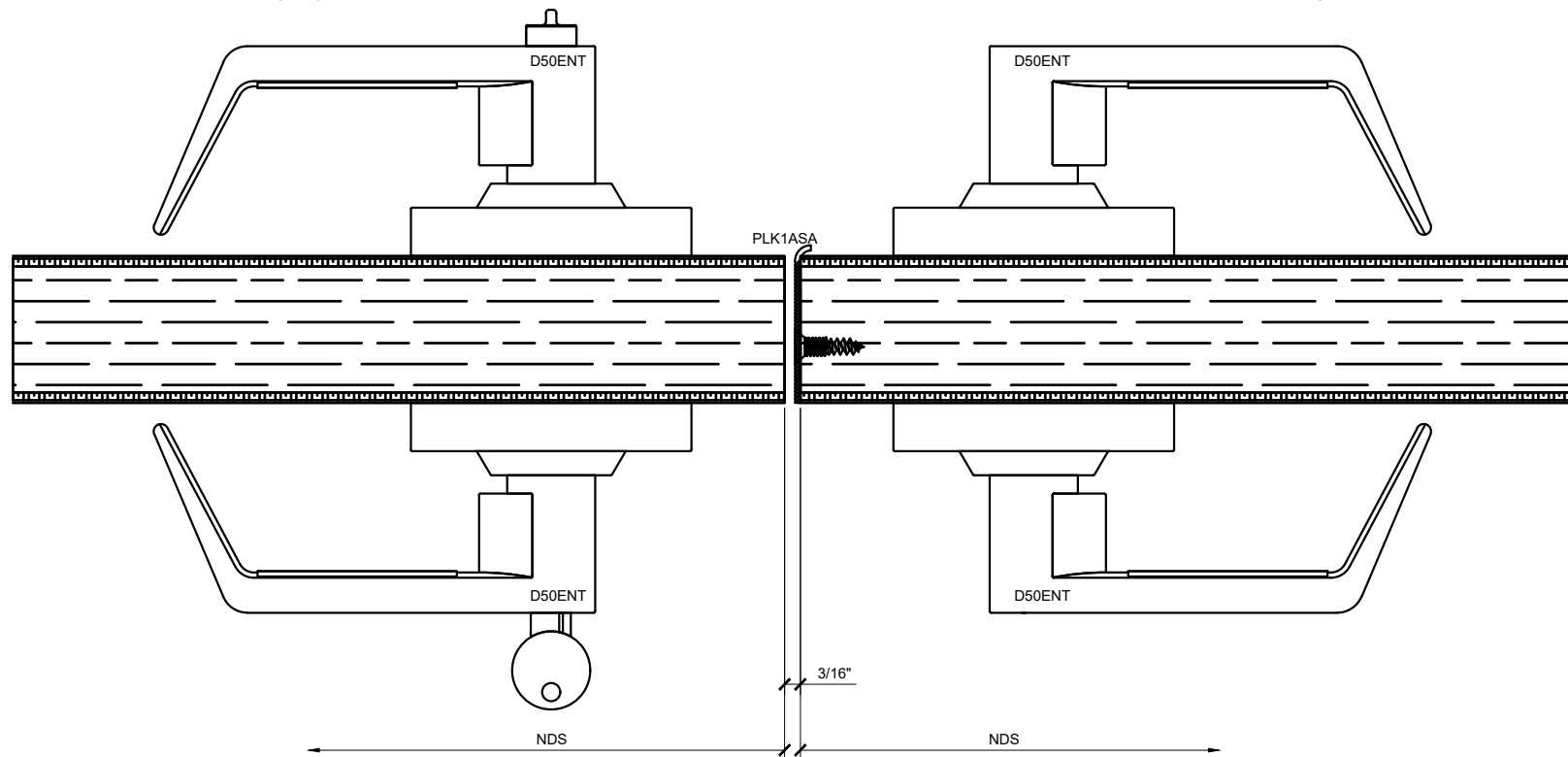
② MEETING STILES DETAIL WITH WOOD FLUSH DOOR
