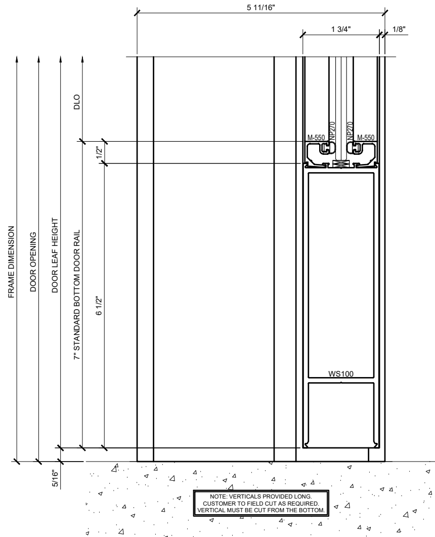
① DOOR SILL DETAIL WITH SERIES 550 WIDE STILE DOOR
