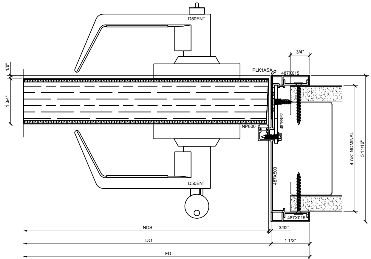
③ DOOR JAMB DETAIL AT STRIKE SIDE WITH WOOD FLUSH DOOR
