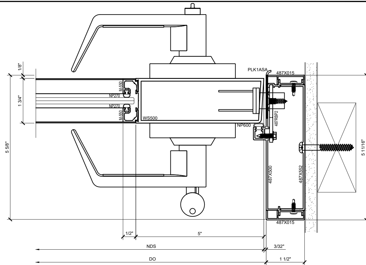
② SURFACE MOUNT DOOR JAMB DETAIL AT STRIKE SIDE W/ SERIES 550 WIDE STILE DOOR ARCH REF: 1'-0"=1'-0"
