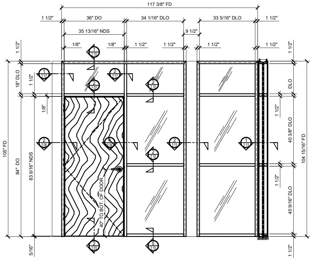
① ELEVATION: WOOD DOOR WITH FULL HEIGHT SIDELITES AND TRANSOMS ARCH REF: NONE 3/4"=1'-0"
