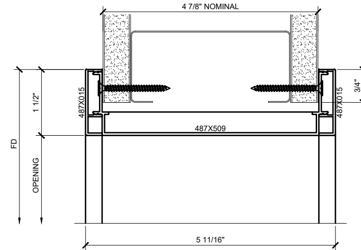
③ HEAD DETAIL AT CASSED OPENING ARCH REF: 1'-0"=1'-0"
