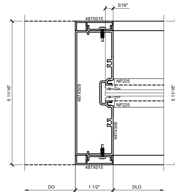
④ CASSED OPENING JAMB DETAIL AT SIDELITE
