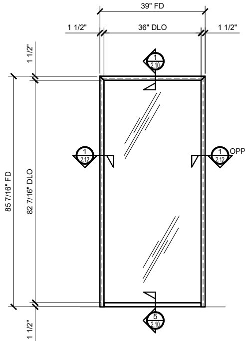
① ELEVATION: BORROWED LITE TO FLOOR ARCH REF: NONE 3/4"=1'-0"
