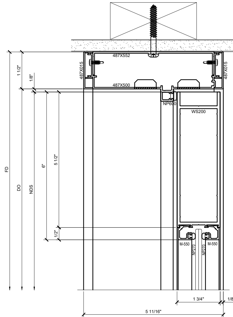
③ SURFACE MOUNTED DOOR HEAD DETAIL WITH SERIES 550 WIDE STILE DOOR
