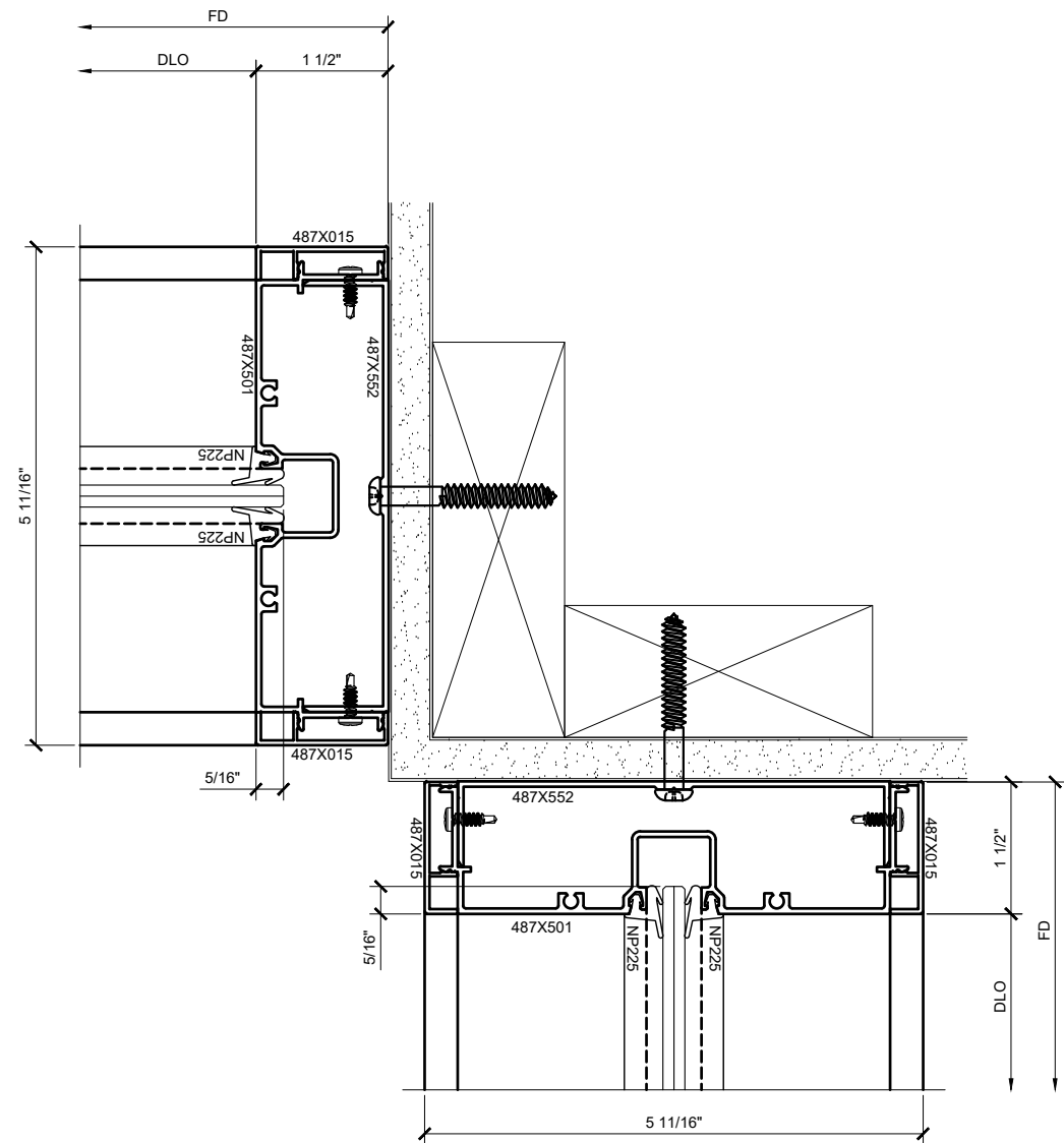
② SURFACE MOUNT CORNER DETAIL: SIDELITE / BORROWED LITE ARCH REF: 1'-0"=1'-0"
