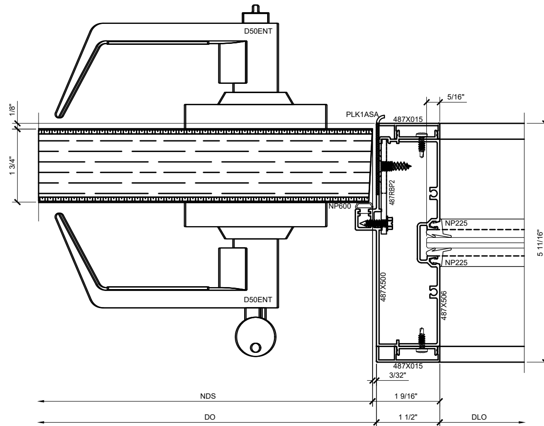
④ DOOR JAMB DETAIL AT STRIKE SIDE WITH SIDELITE W/ WOOD FLUSH DOOR ARCH REF: 1'-0"=1'-0"
