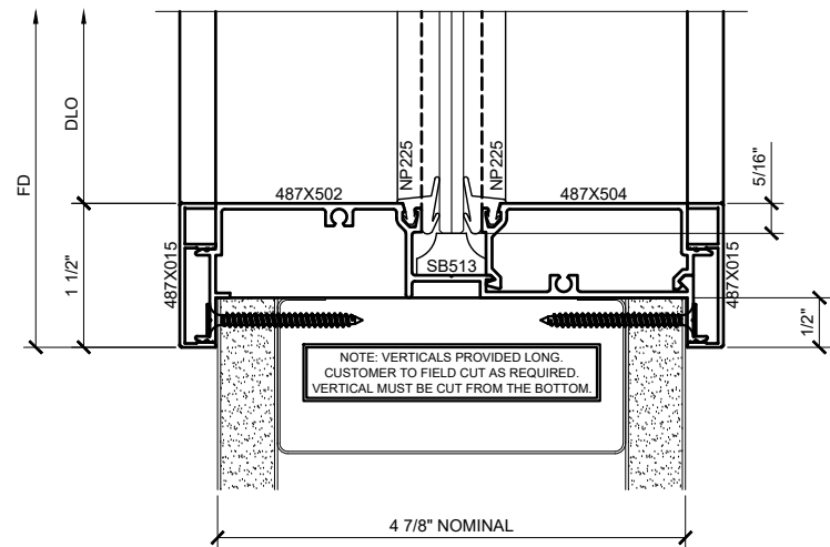
④ SILL DETAIL AT SIDELITE / BORROWED LITE ABOVE FLOOR ARCH REF: 1'-0"=1'-0"
