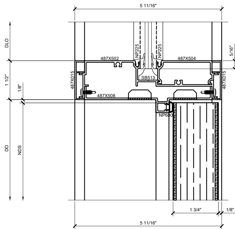
② DOOR HEAD DETAIL AT TRANSOM WITH WOOD FLUSH DOOR
