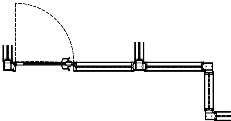
①A PLAN VIEW ARCH REF: NONE 3/4"=1'-0"
