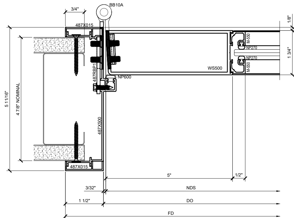
① DOOR JAMB DETAIL AT HINGE SIDE WITH SERIES 550 WIDE STILE DOOR ARCH REF: 1'-0\"=1'-0\"
