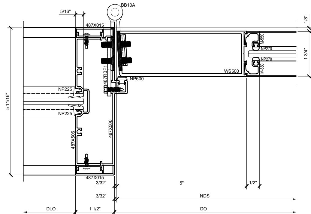
① DOOR JAMB DETAIL AT HINGE SIDE WITH SIDELITE W/ SERIES 550 WIDE STILE DOOR ARCH REF: 1'-0"=1'-0"
