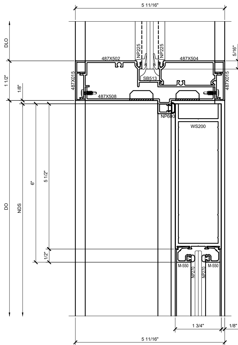
② DOOR HEAD DETAIL AT TRANSOM WITH SERIES 550 WIDE STILE DOOR
