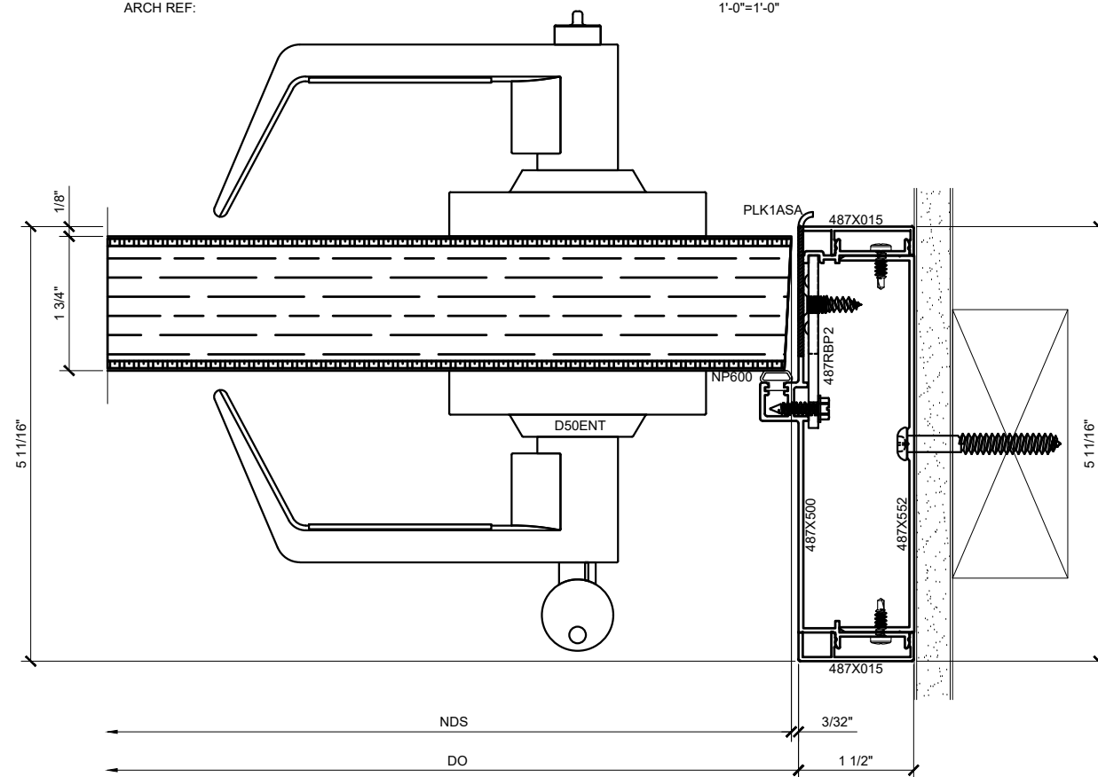
④ SURFACE MOUNT DOOR JAMB DETAIL AT STRIKE SIDE WITH WOOD FLUSH DOOR ARCH REF: 1'-0"=1'-0"
