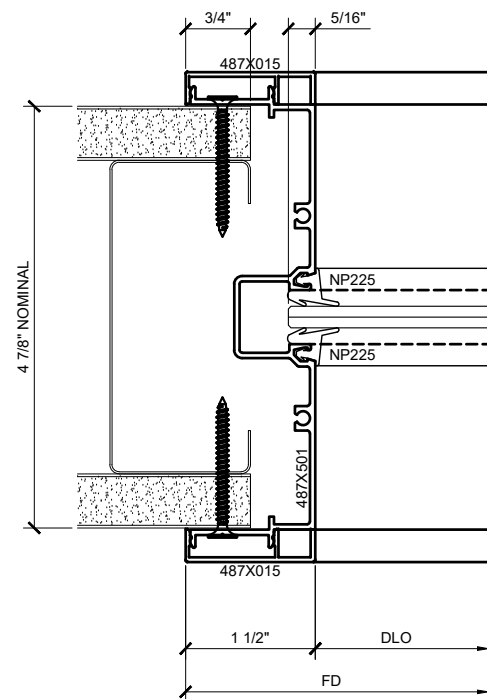
① WALL JAMB DETAIL AT SIDELITE / BORROWED LITE
