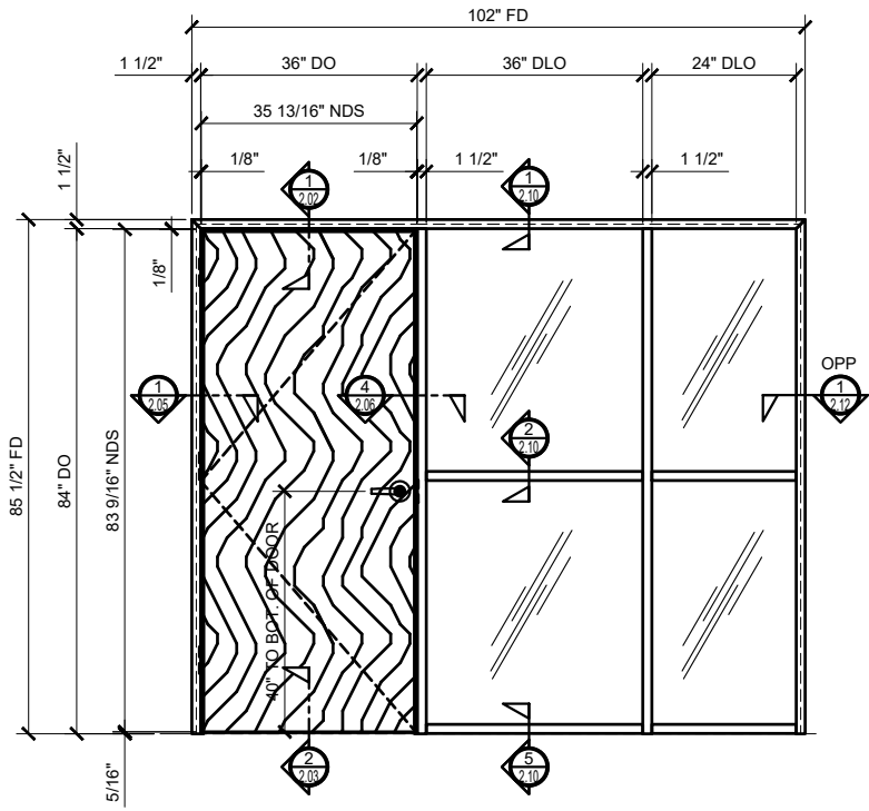
② ELEVATION: WOOD DOOR WITH FULL HEIGHT SIDELITES ARCH REF: NONE 3/4"=1'-0"
