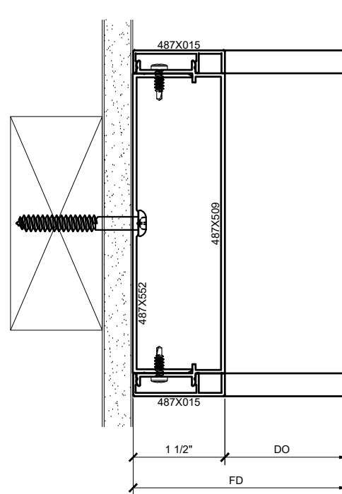
⑥ SURFACE MOUNT WALL JAMB DETAIL AT CASSED OPENING
