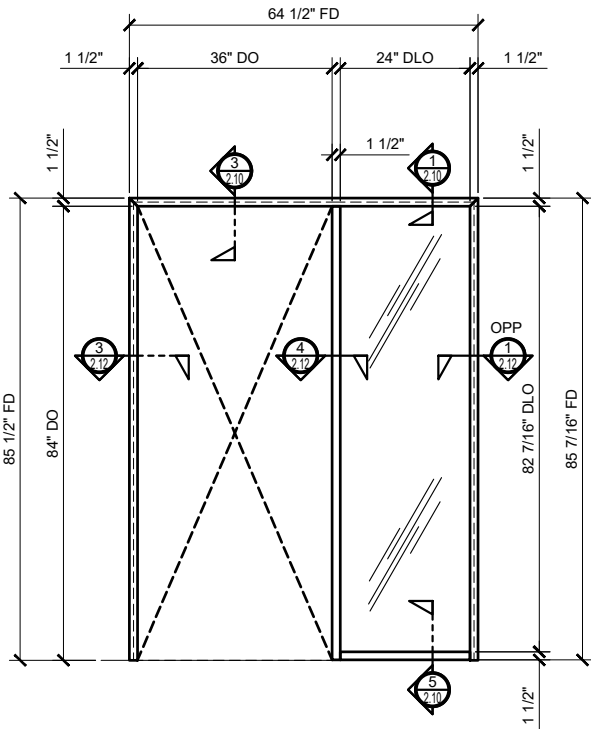
① ELEVATION: SINGLE CASSED OPENING WITH FULL HEIGHT SIDELITE ARCH REF: NONE 3/4"=1'-0"
