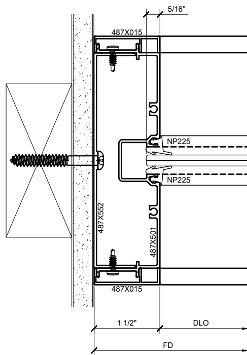
⑤ SURFACE MOUNT WALL JAMB DETAIL AT SIDELITE / BORROWED LITE
