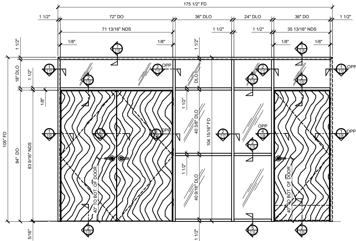
① ELEVATION: WOOD DOORS WITH FULL HEIGHT SIDELITES AND TRANSOMS ARCH REF: NONE 3/4"=1'-0"
