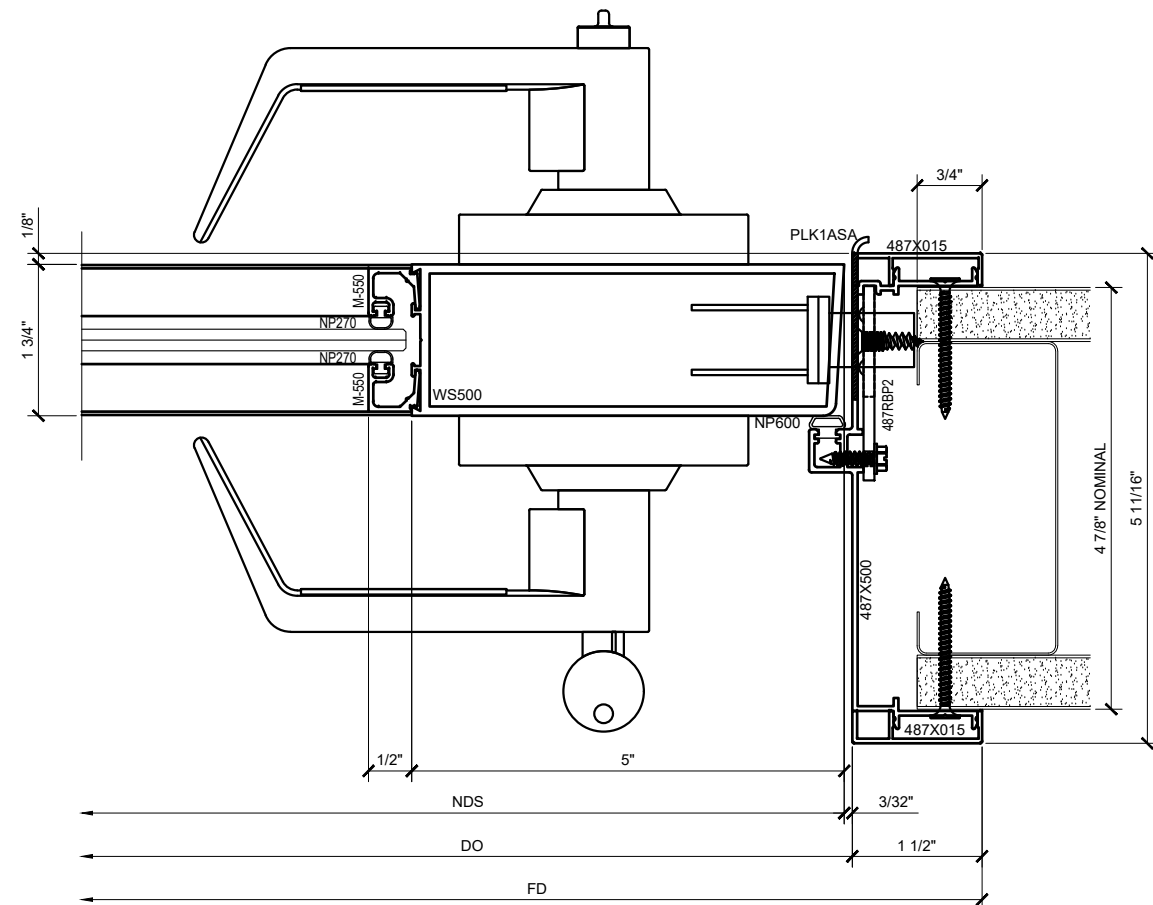
③ DOOR JAMB DETAIL AT STRIKE SIDE WITH SERIES 550 WIDE STILE DOOR ARCH REF: 1'-0\"=1'-0\"
