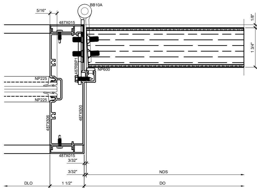
③ DOOR JAMB DETAIL AT HINGE SIDE WITH SIDELITE W/ WOOD FLUSH DOOR ARCH REF: 1'-0"=1'-0"
