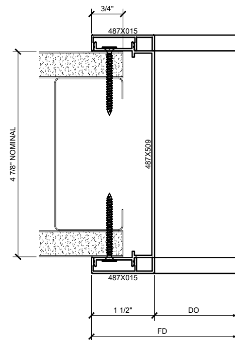
③ WALL JAMB DETAIL AT CASSED OPENING
