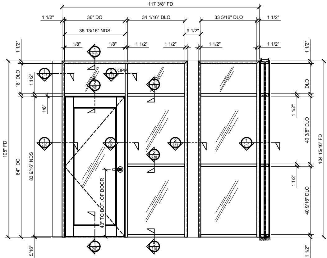
① ELEVATION: ALUMINUM DOOR WITH FULL HEIGHT SIDELITES AND TRANSOMS ARCH REF: NONE 3/4"=1'-0"
