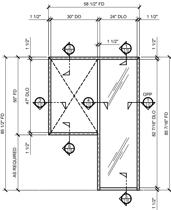
② ELEVATION: SINGLE CASSED OPENING ABOVE FLOOR WITH FULL HEIGHT SIDELITE ARCH REF: NONE 3/4"=1'-0"
