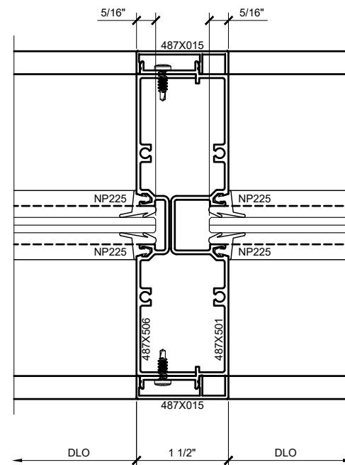
② INTERMEDIATE VERTICAL DETAIL AT SIDELITE
