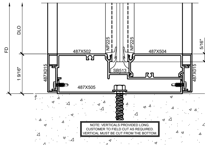
⑤ SILL DETAIL AT FULL HEIGHT SIDELITE / BORROWED LITE ARCH REF: 1'-0"=1'-0"
