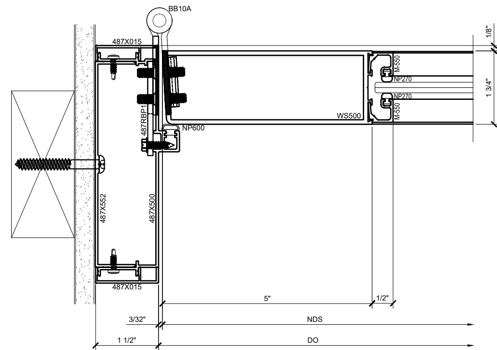
① SURFACE MOUNT DOOR JAMB DETAIL AT HINGE SIDE W/ SERIES 550 WIDE STILE DOOR ARCH REF: 1'-0"=1'-0"
