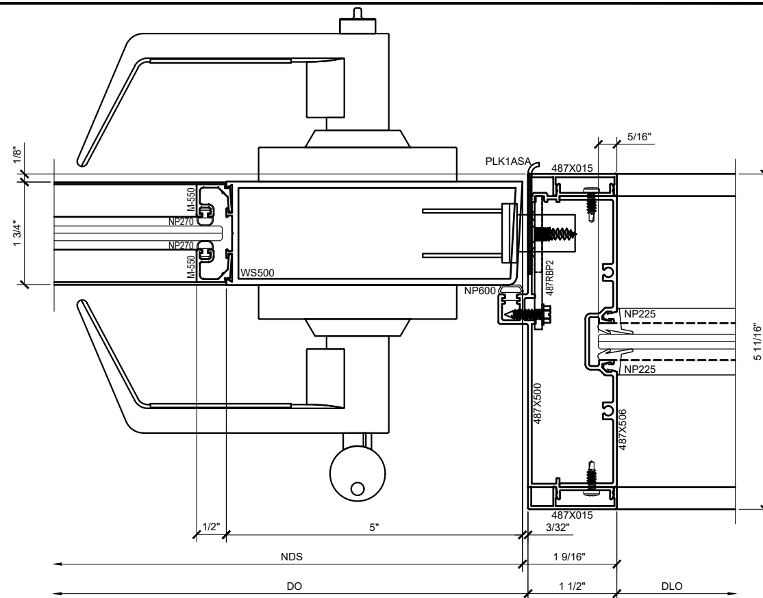
② DOOR JAMB DETAIL AT STRIKE SIDE WITH SIDELITE W/SERIES 550 WIDE STILE DOOR ARCH REF: 1'-0"=1'-0"
