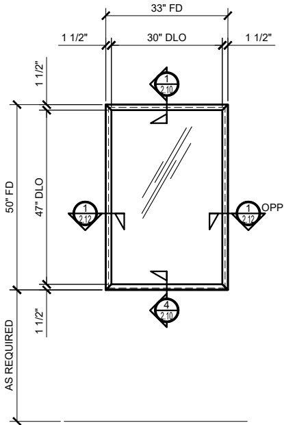
② ELEVATION: BORROWED LITE ABOVE FLOOR ARCH REF: NONE 3/4"=1'-0"
