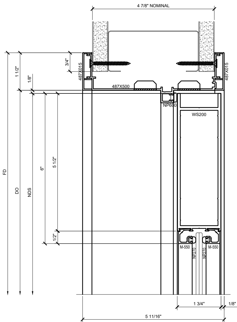
① DOOR HEAD DETAIL WITH SERIES 550 WIDE STILE DOOR
