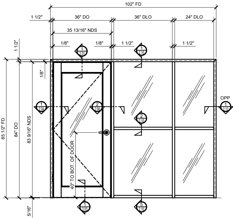
② ELEVATION: ALUMINUM DOOR WITH FULL HEIGHT SIDELITES ARCH REF: NONE 3/4"=1'-0"
