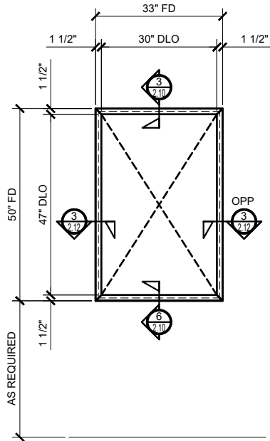
④ ELEVATION: SINGLE CASSED PASS-THRU ARCH REF: NONE 3/4"=1'-0"
