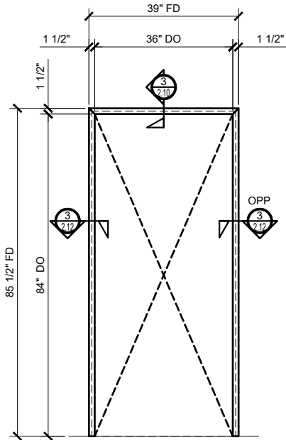
③ ELEVATION: SINGLE CASSED OPENING ARCH REF: NONE 3/4"=1'-0"
