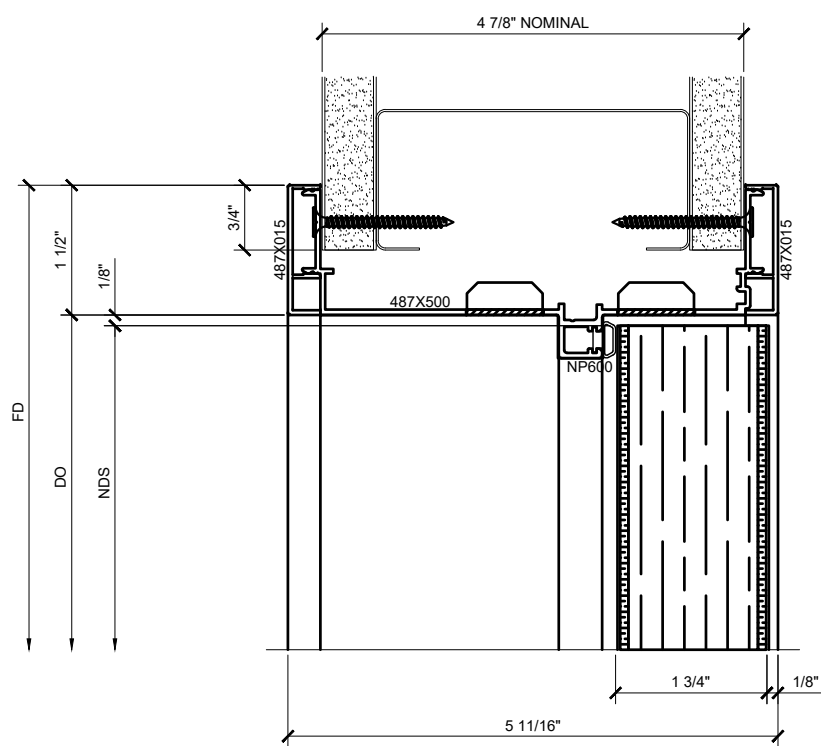
① DOOR HEAD DETAIL WITH WOOD FLUSH DOOR
