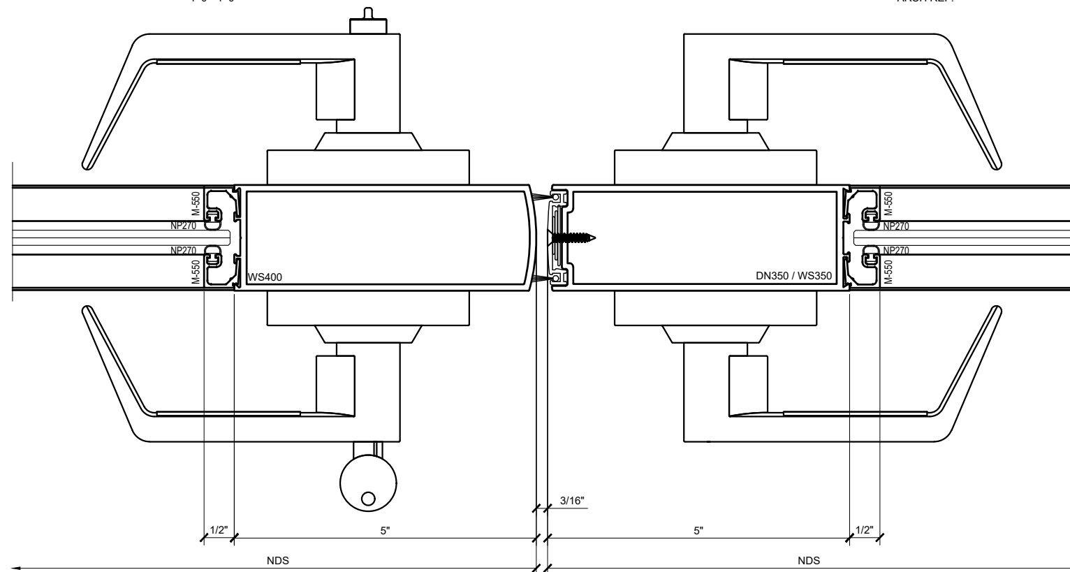
② MEETING STILES DETAIL WITH SERIES 550 WIDE STILE DOORS ARCH REF: 1'-0\"=1'-0\"
