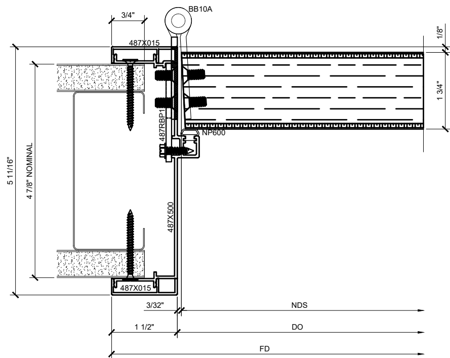
① DOOR JAMB DETAIL AT HINGE SIDE WITH WOOD FLUSH DOOR
